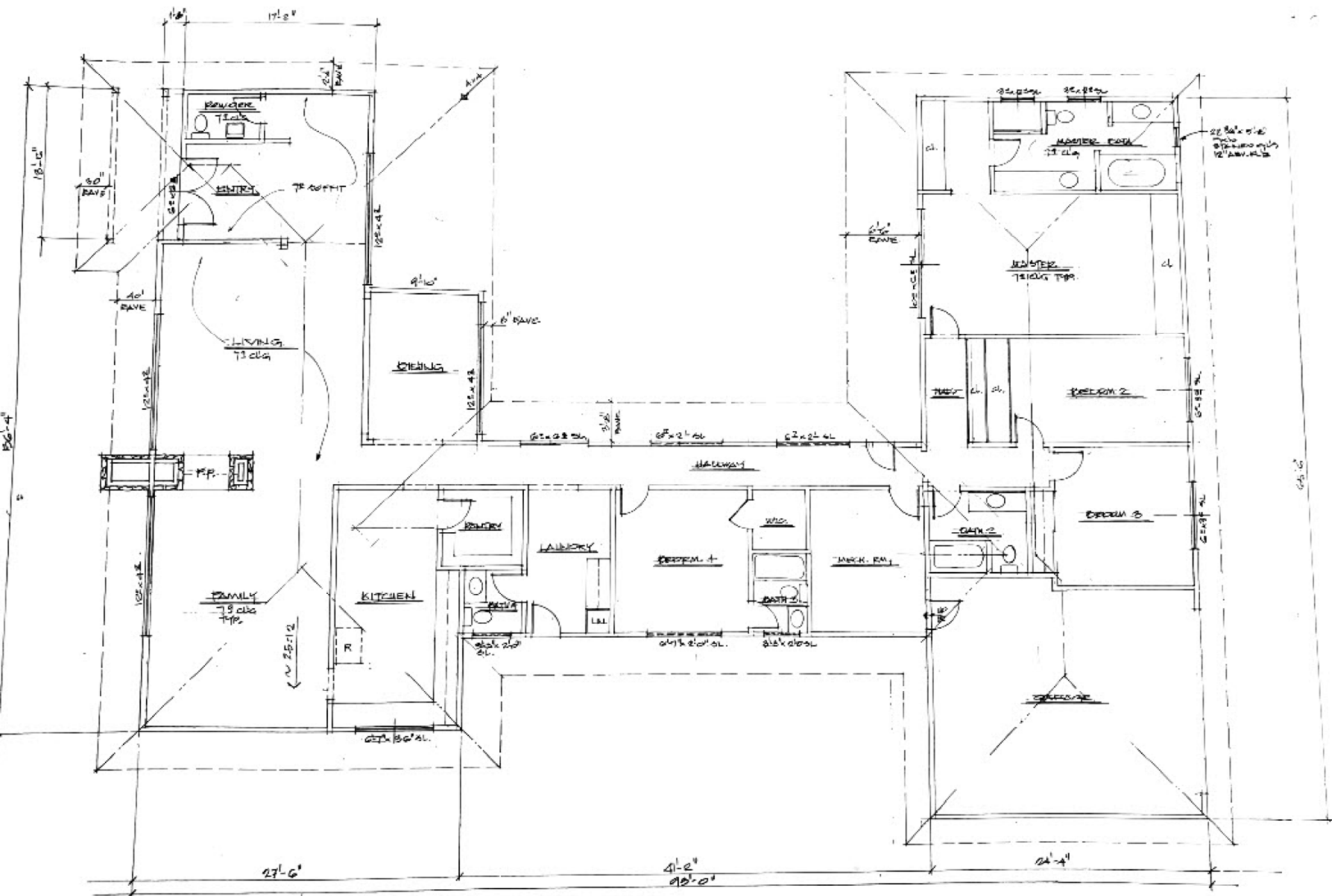
AS BUILT FLOOR PLAN BR. 1/4" = 1/10"
