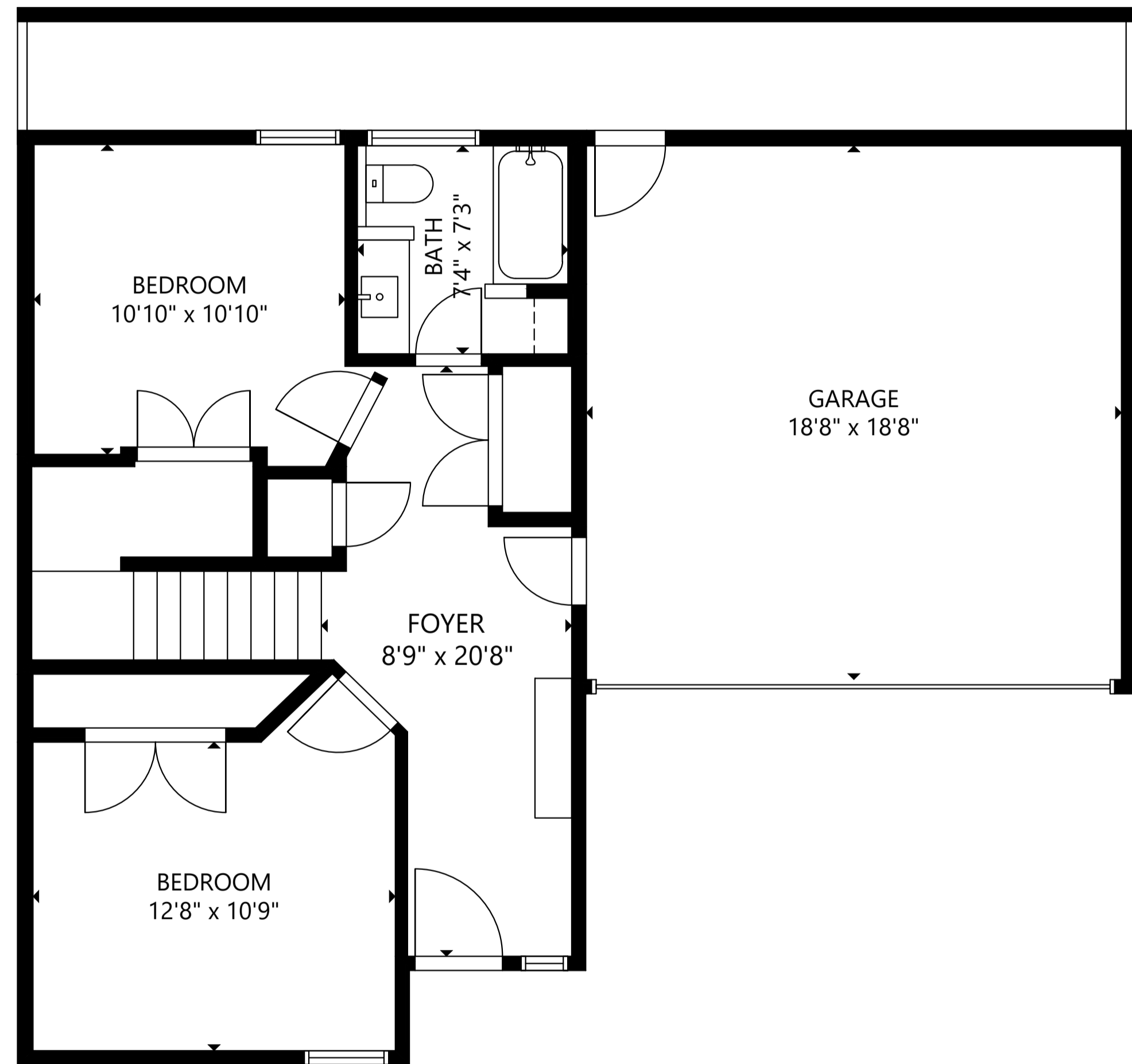
FLOOR 1
