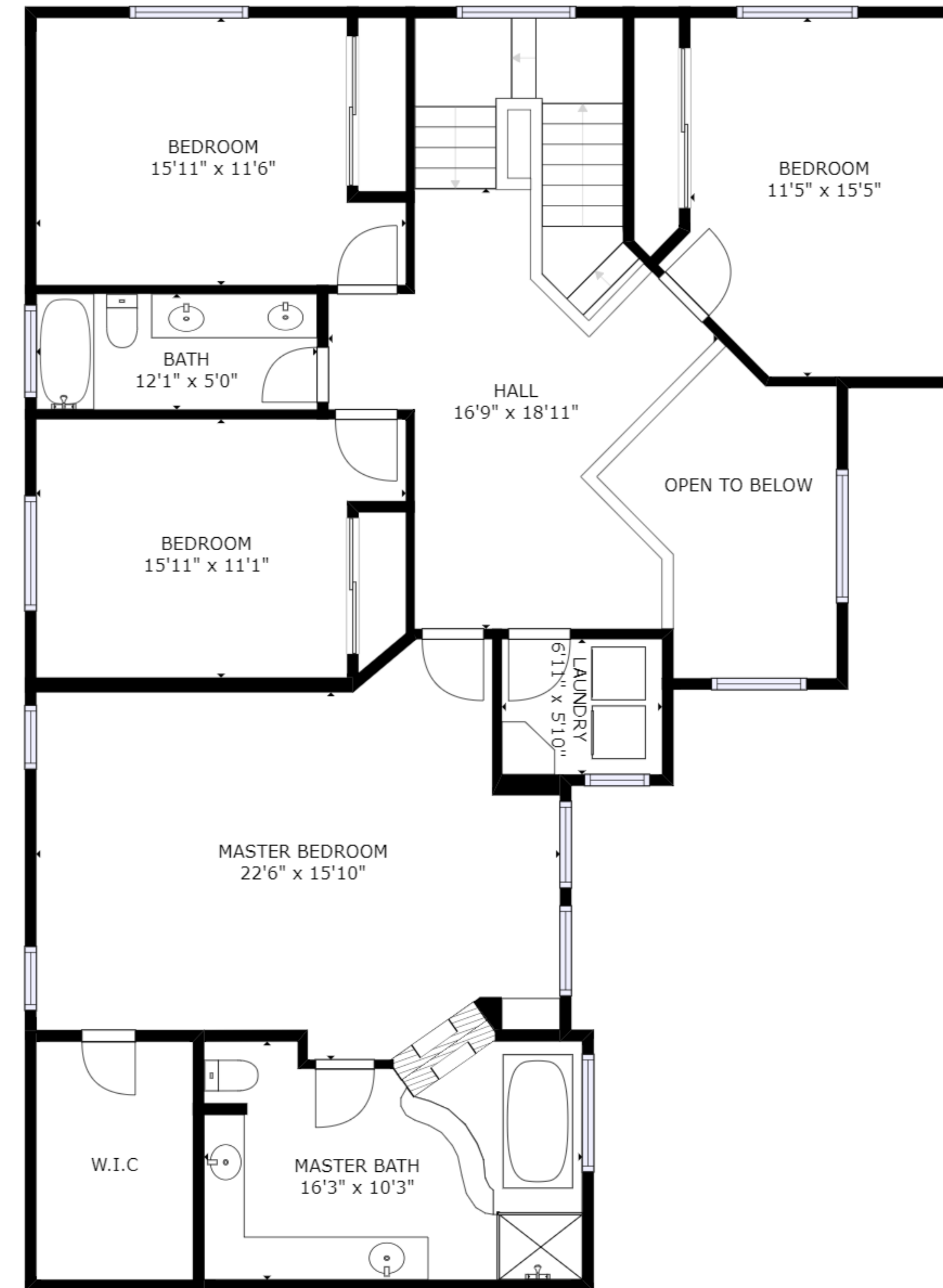
FLOOR 2
