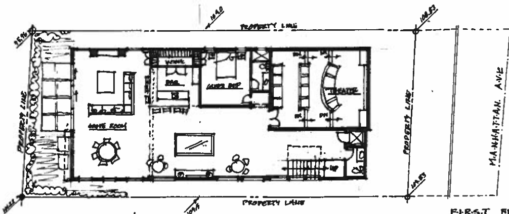
FIRST FLOOR (2240 SQ. FT.)
