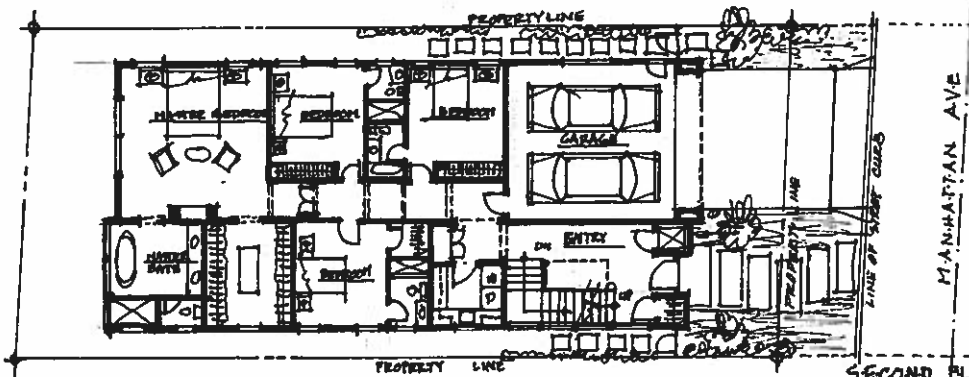
SECOND FLOOR (1722 SQ. FT.)
