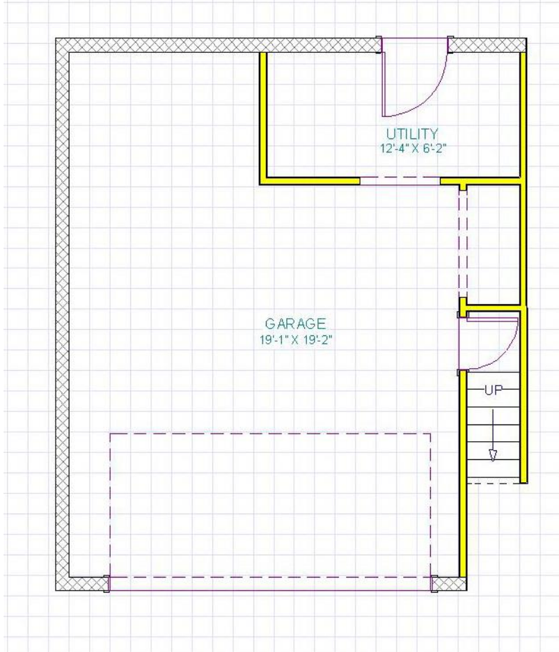
Level 1 – Garage and Laundry
