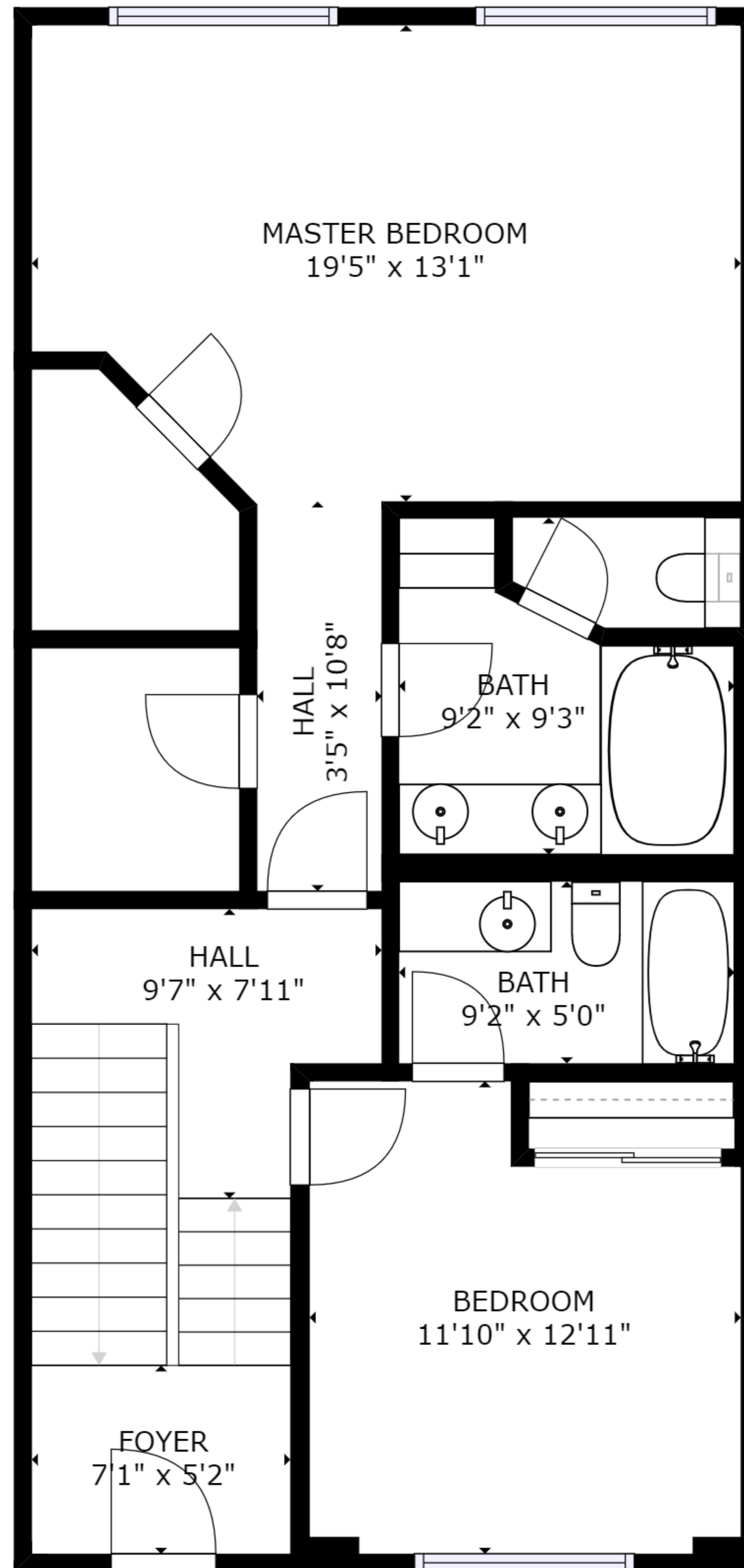
FLOOR 2
