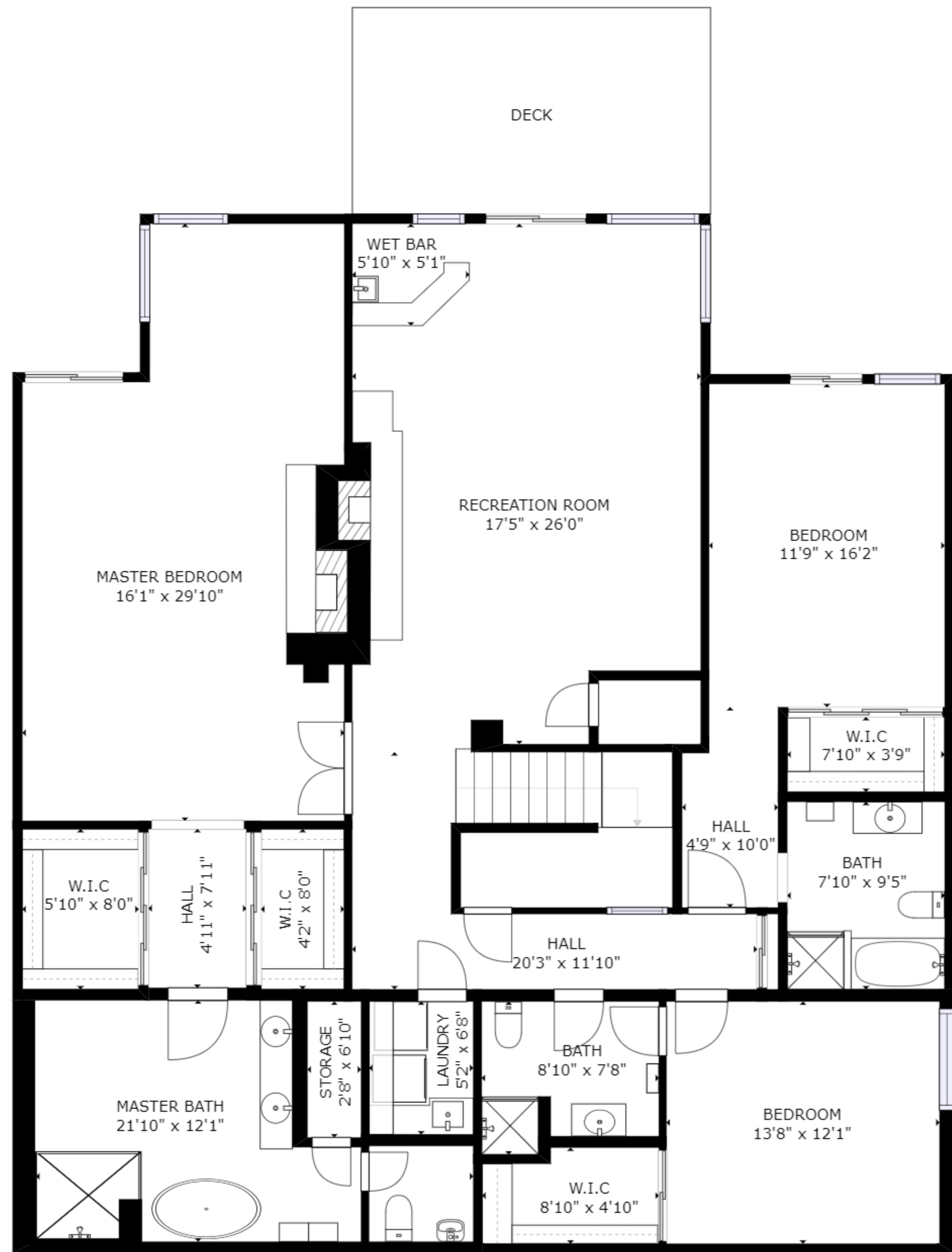
FLOOR 1
