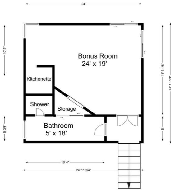
Lower Floor
