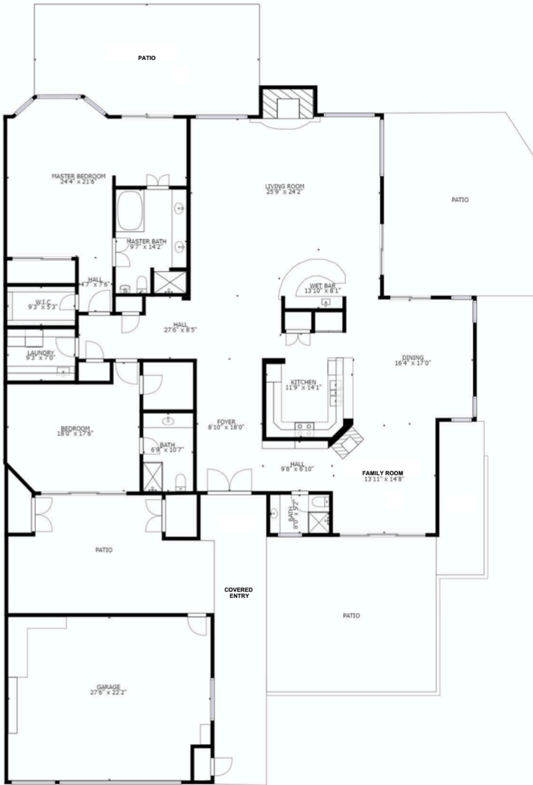
FLOOR 1
