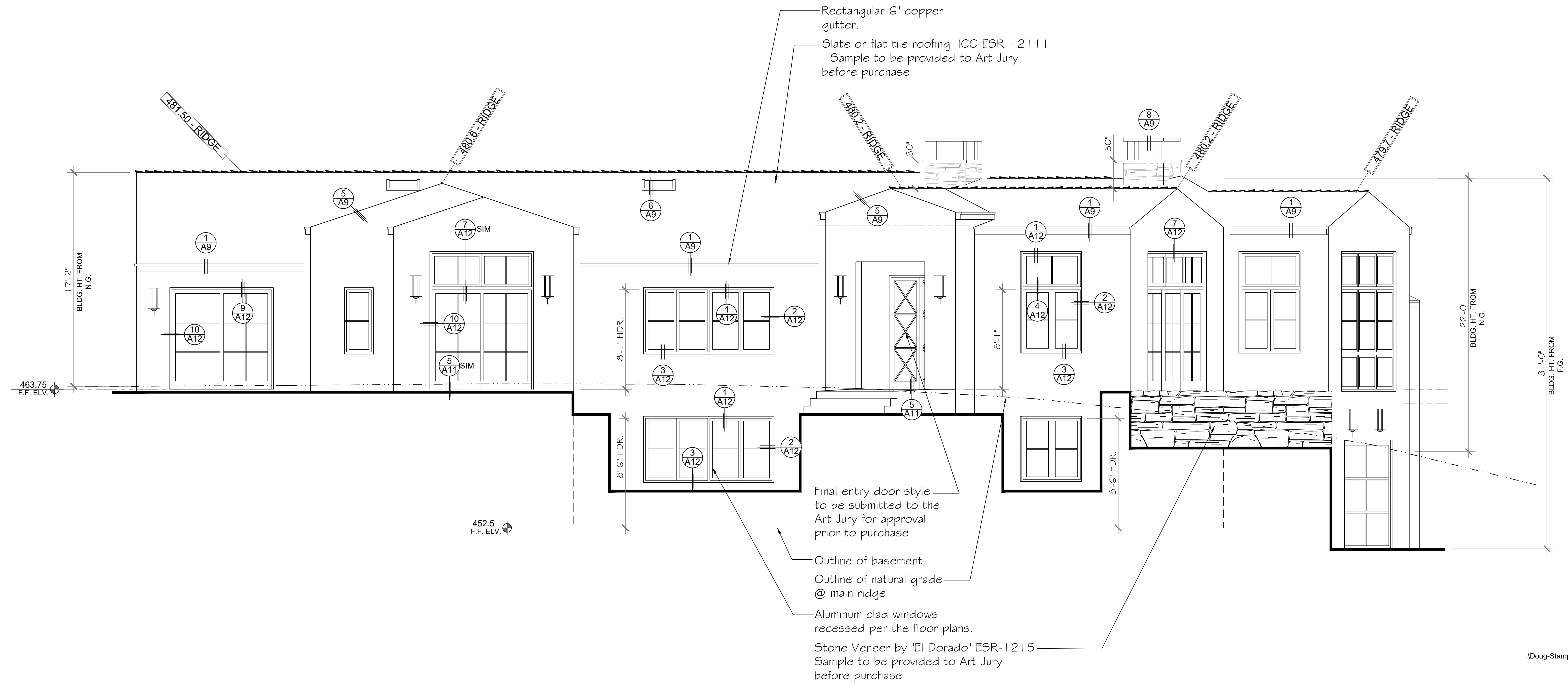
VIA HORQUILLA EAST ELEVATION 1/4" = 1'-0"
