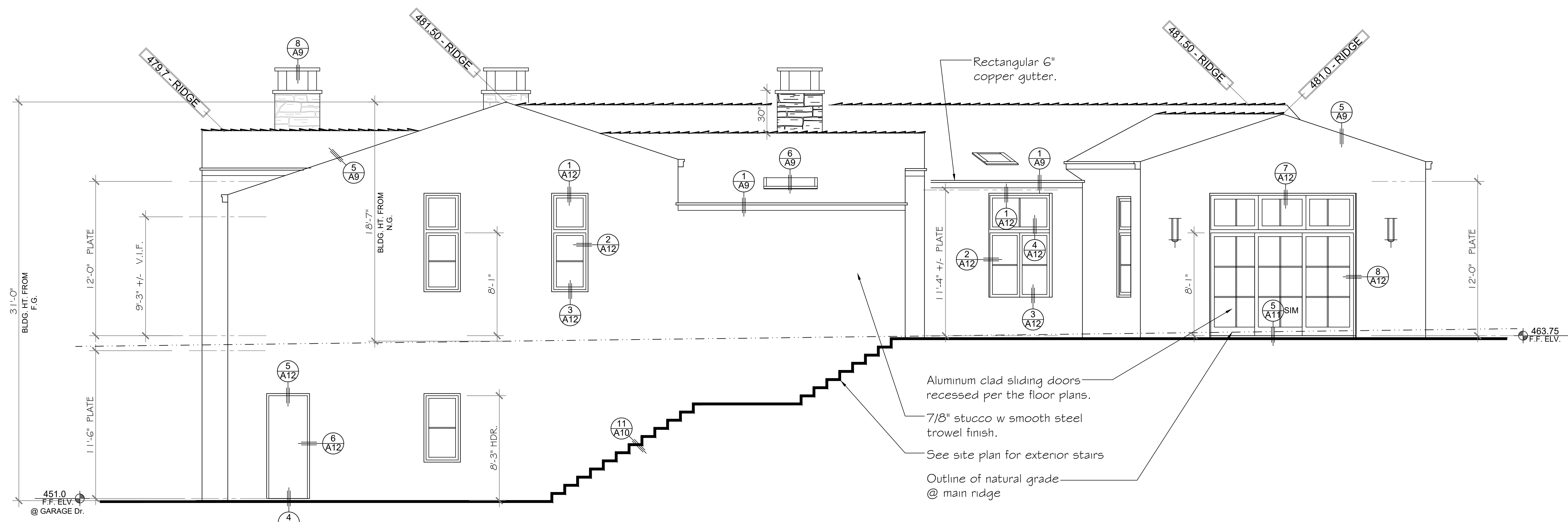
SIDE WEST ELEVATION 1/4" = 1'-0"
