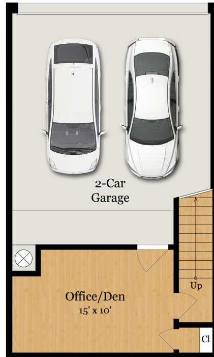
LOWER LEVEL 235 SQ FT
