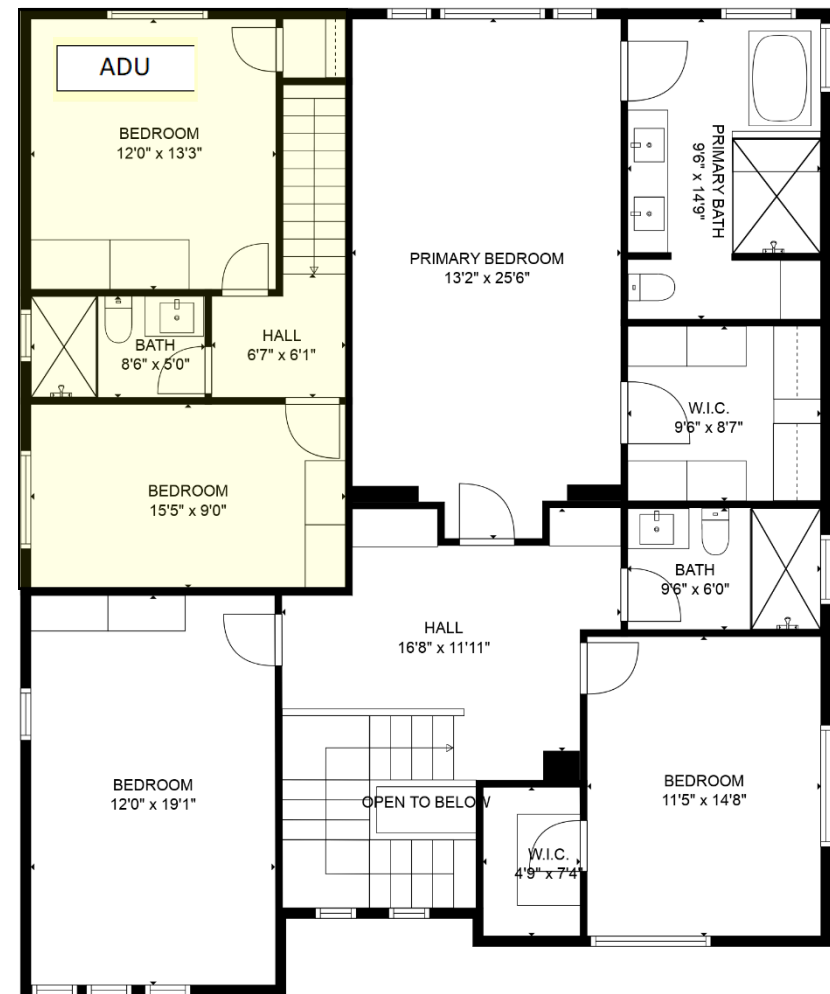
FLOOR 2
