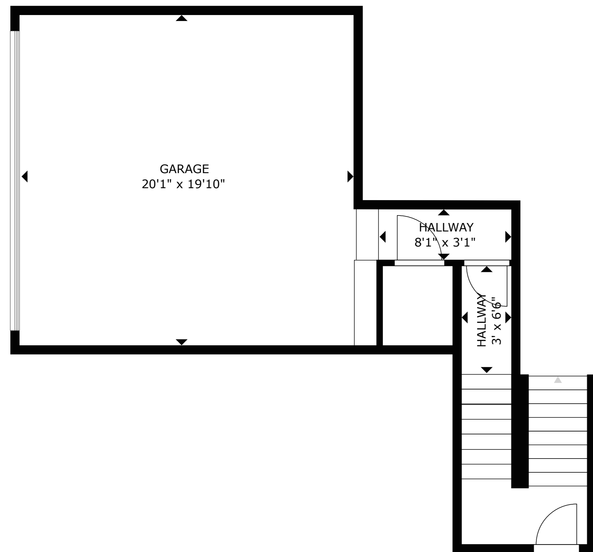
FLOOR 1
