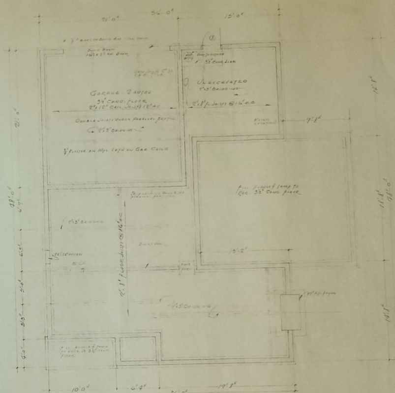
FOUNDATION & GARAGE PLAN
