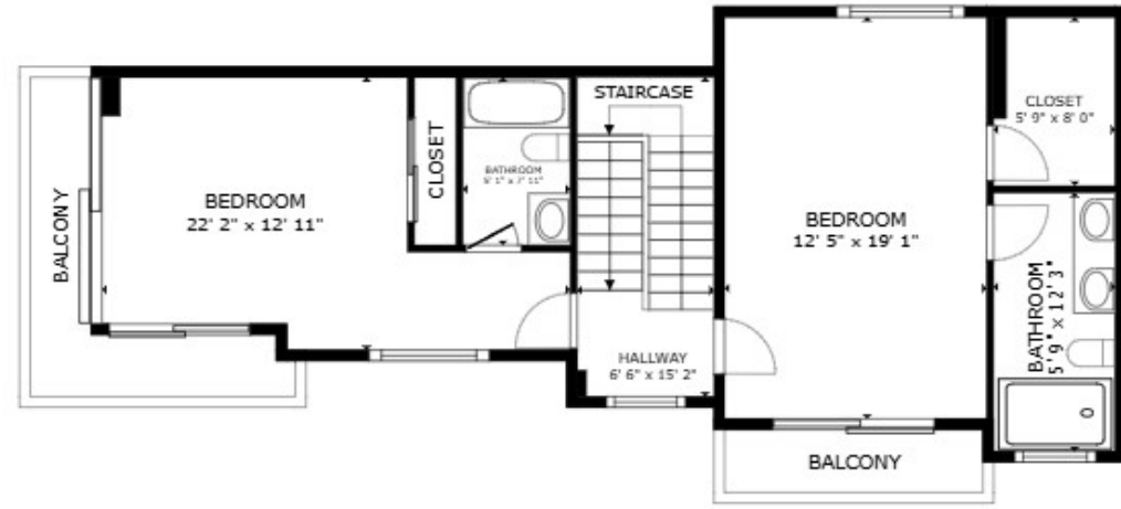
FLOOR 3
