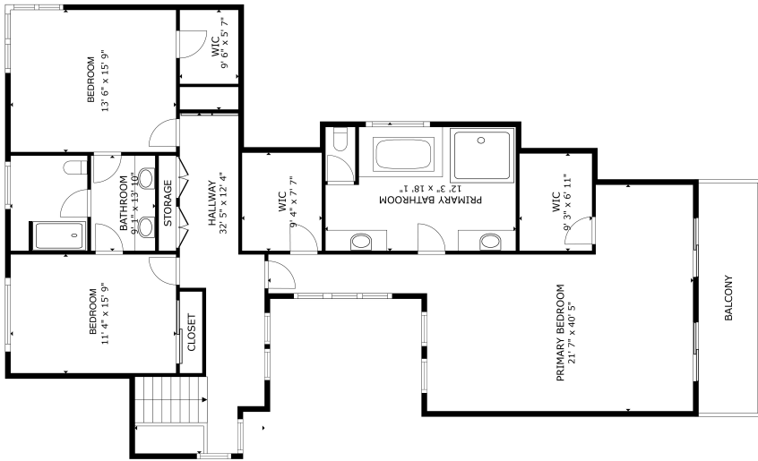
FLOOR 2
