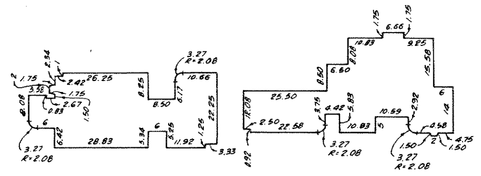
TYPICAL BUILDING DETAILS SCALE 1" = 30'
