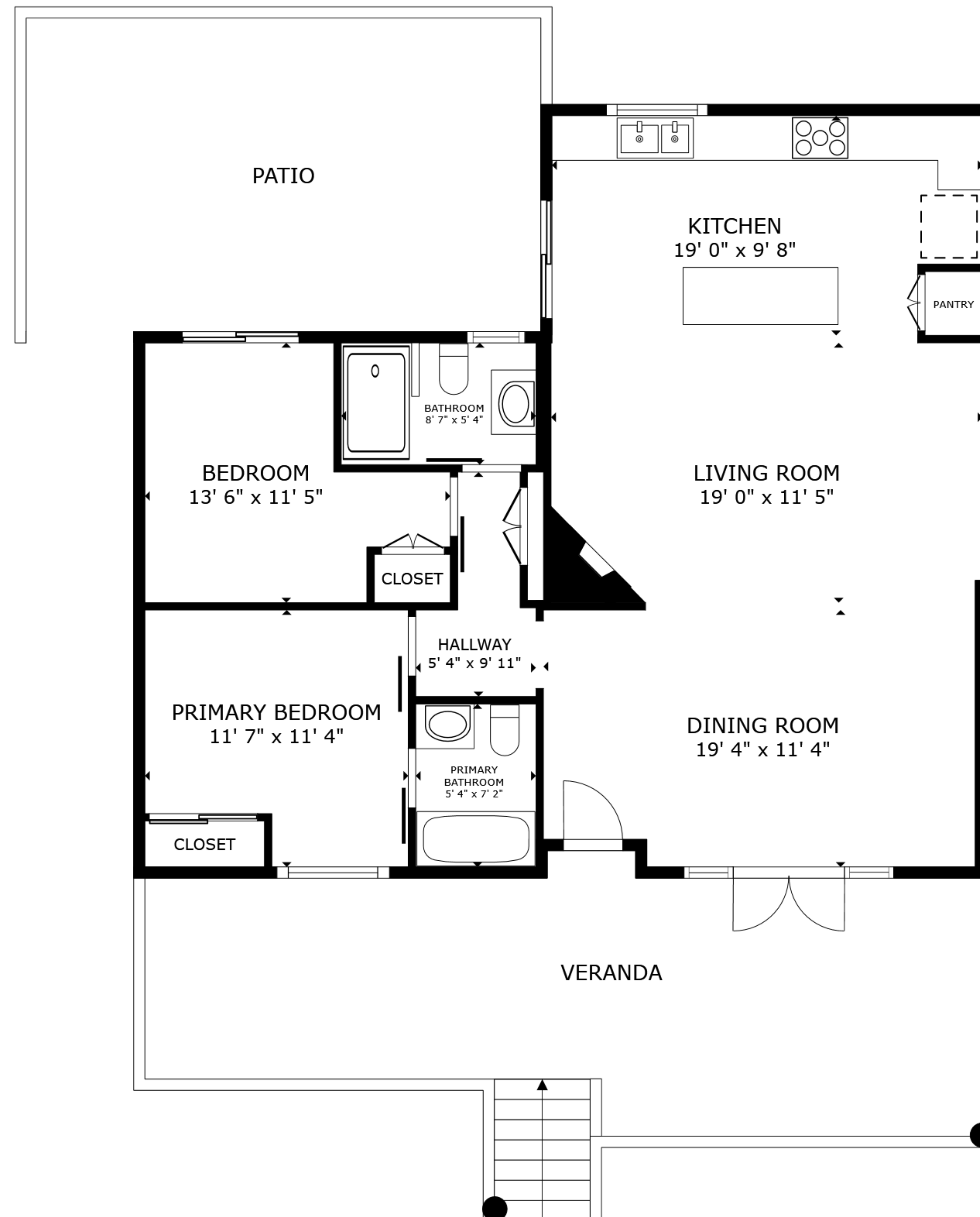
FLOOR PLAN
