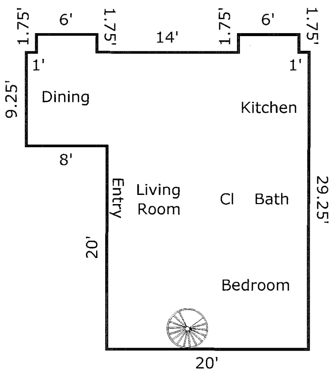
Second Floor [680 Sq ft]
