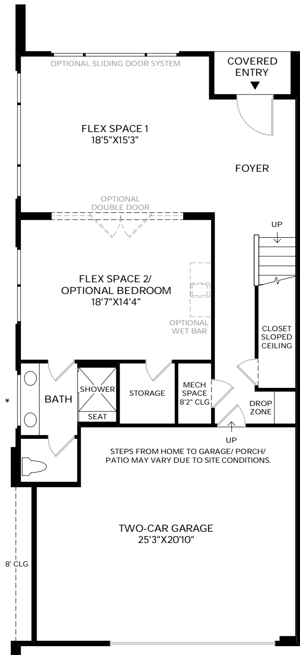
First Floor 9' CEILING HEIGHT
