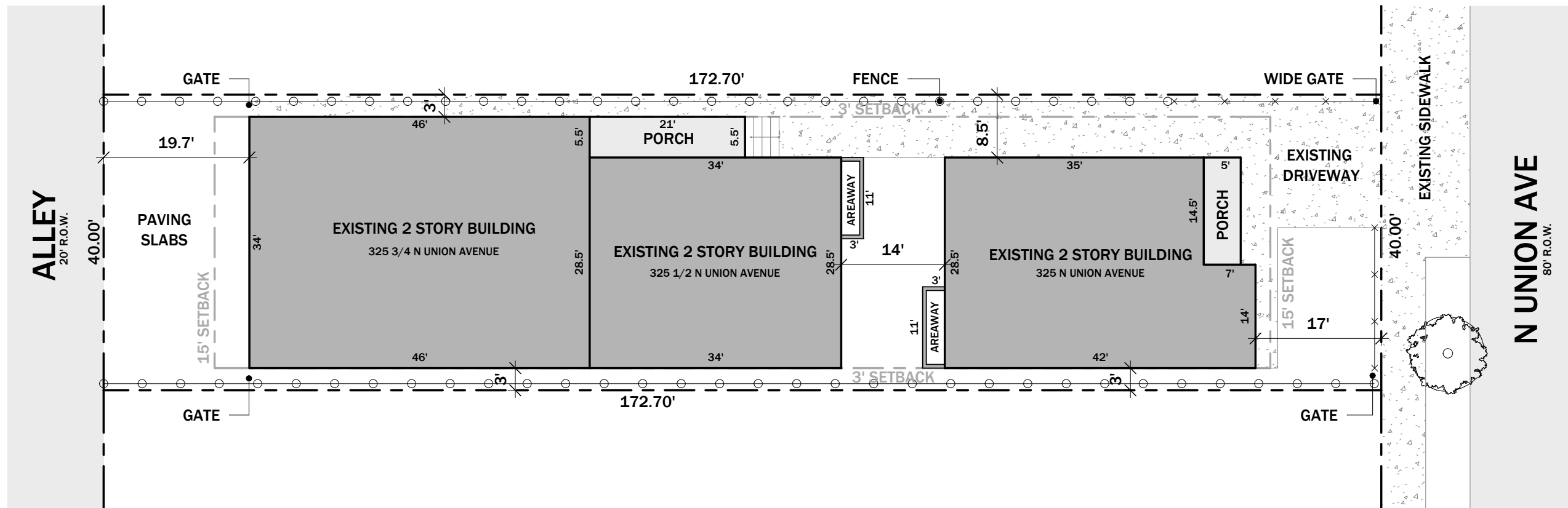
1 SITE PLAN SCALE: 1/16" = 1'-0"
