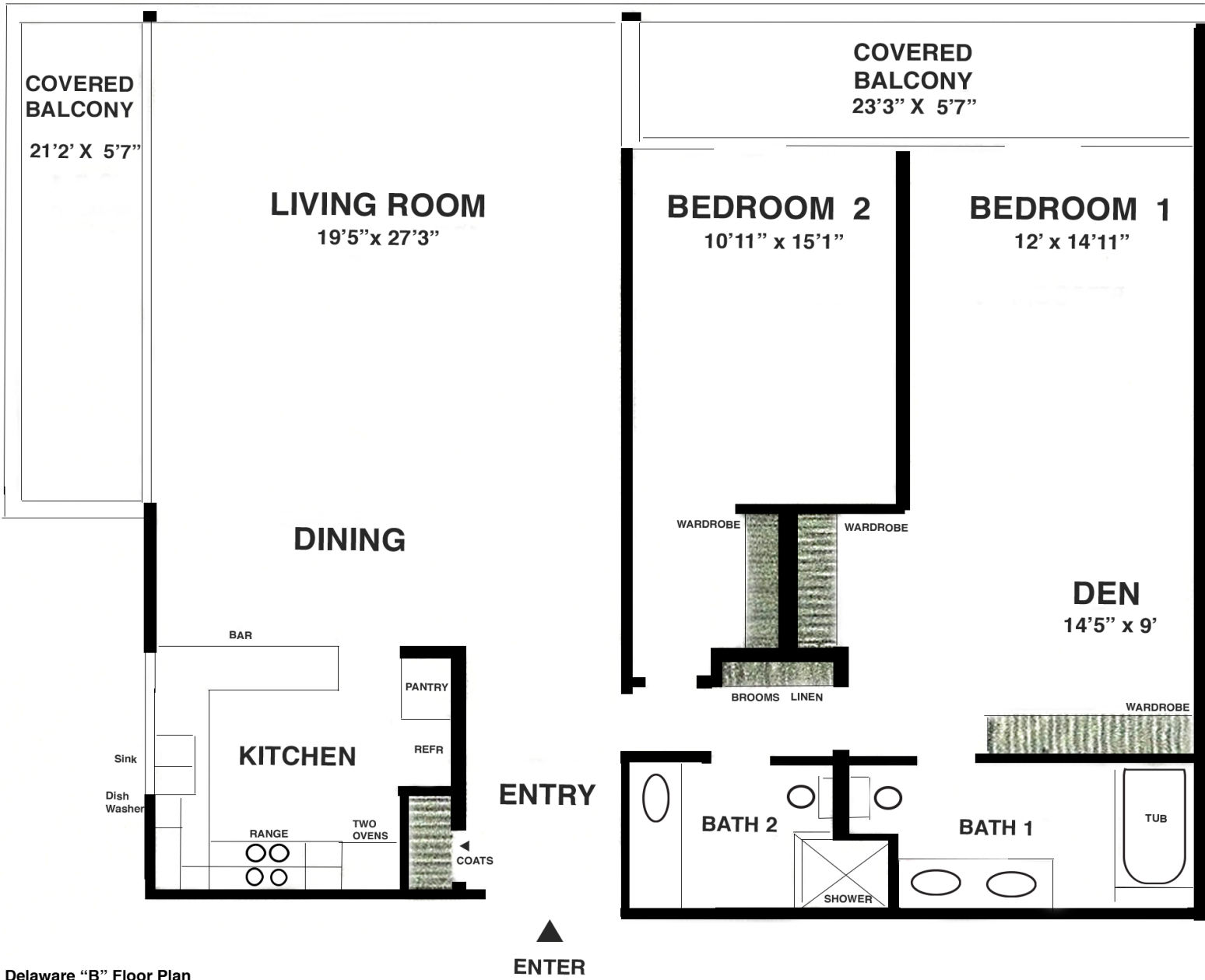
Delaware "B" Floor Plan *Dimensions are approximate unless noted otherwise.
