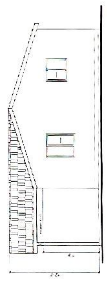
HOUSE ELEVATION SCALE: 1/4" = 1' - 0"
