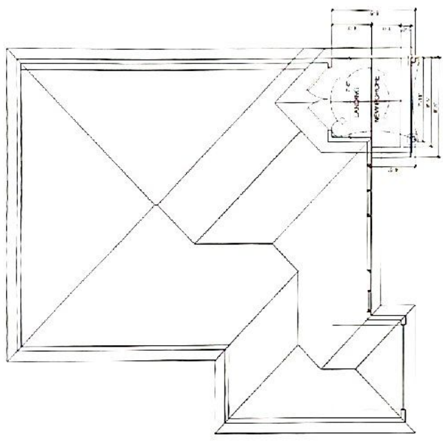
HOUSE WITH NEW PATIO COVER SCALE: 1/4" = 1' - 0"
