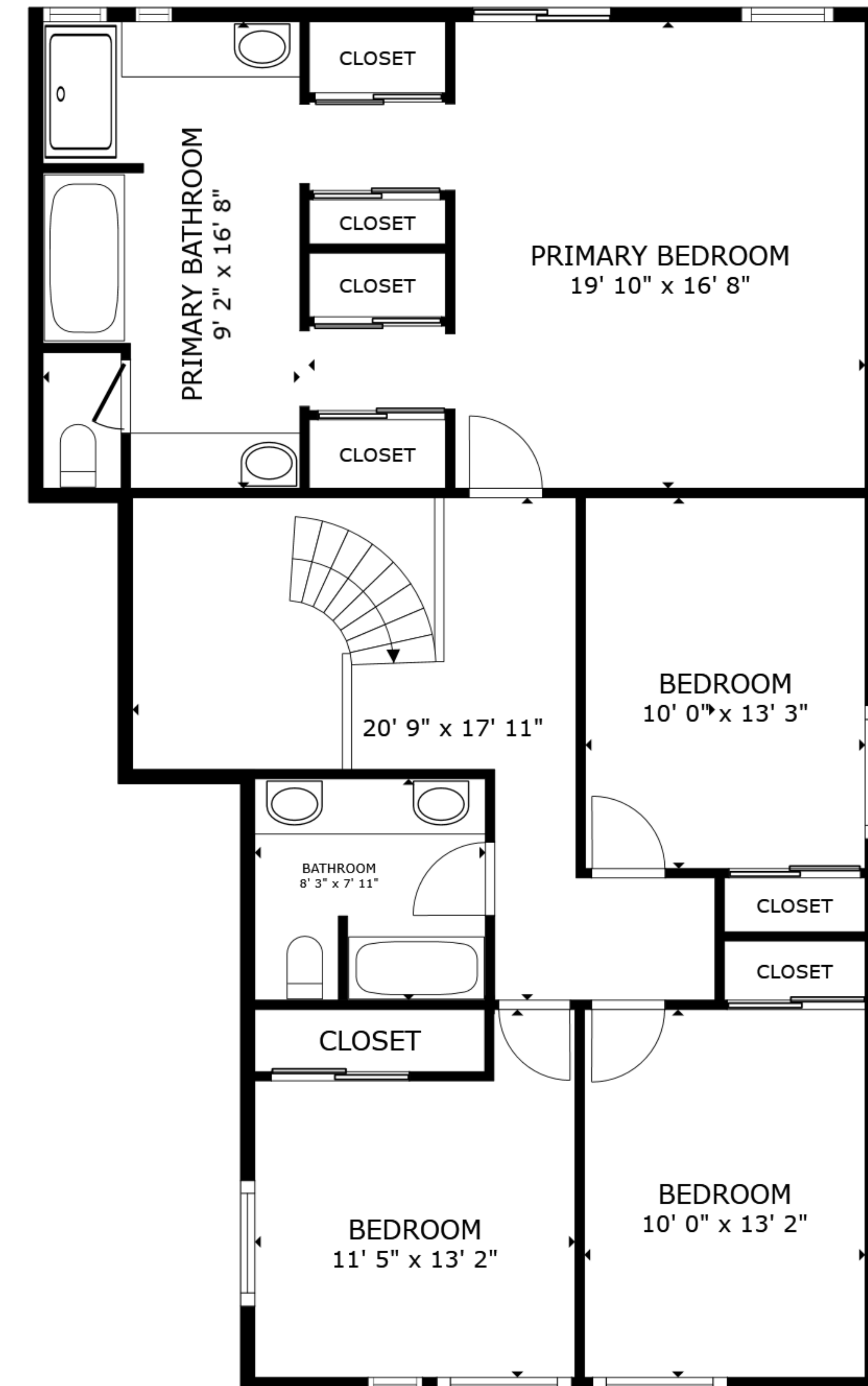
FLOOR 2
