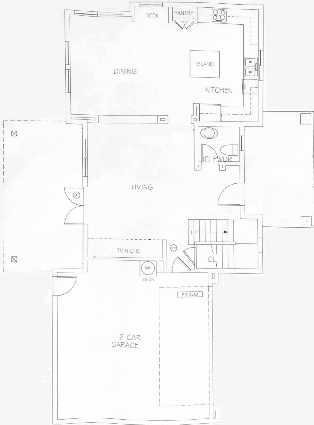
First Floor
