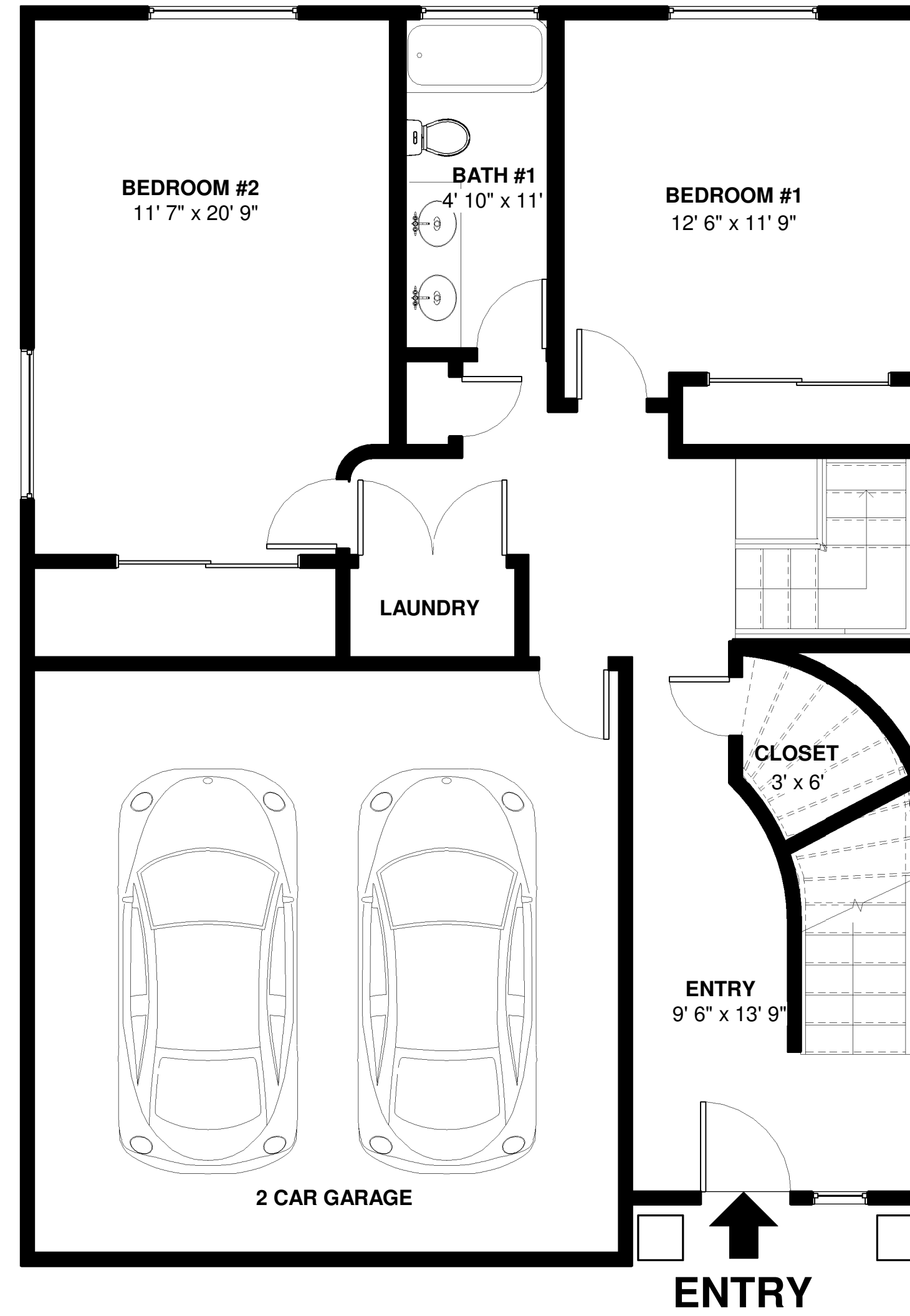
2 FIRST FLOOR 1/4" = 1'-0"
