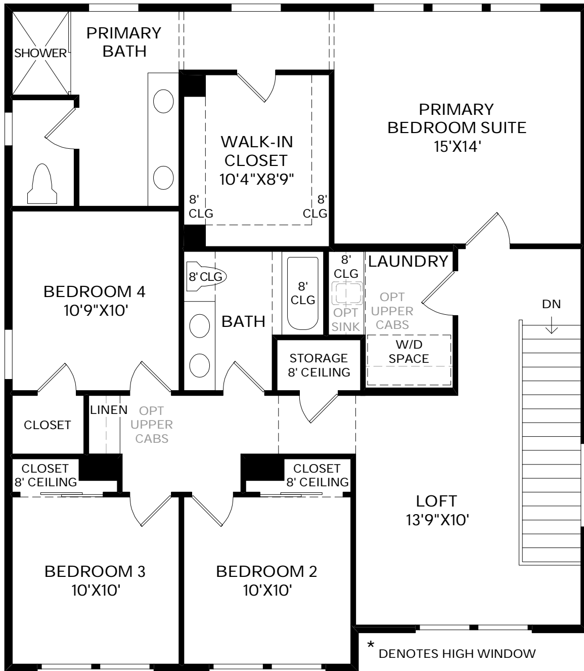
SECOND FLOOR 9' CEILING HEIGHT
