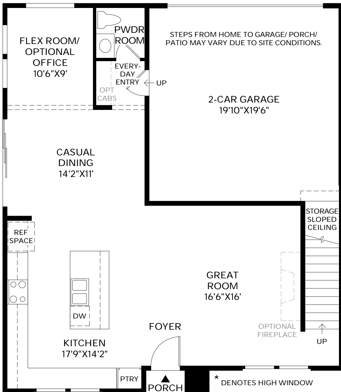
FIRST FLOOR 10' CEILING HEIGHT
