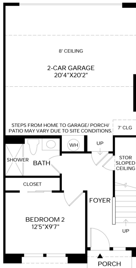
FIRST FLOOR 9' CEILING HEIGHT
