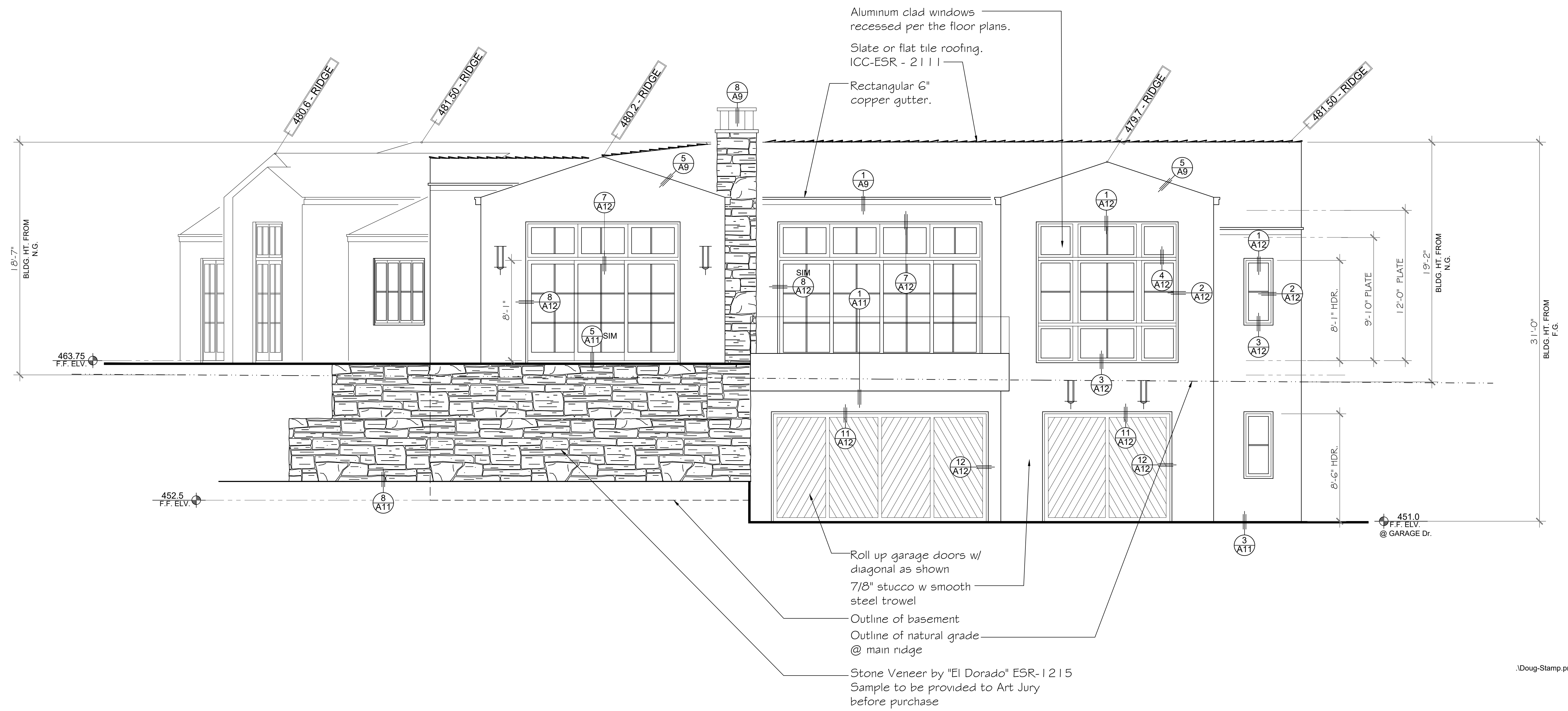
VIA CAMPESINA NORTH ELEVATION 1/4" = 1'-0"
