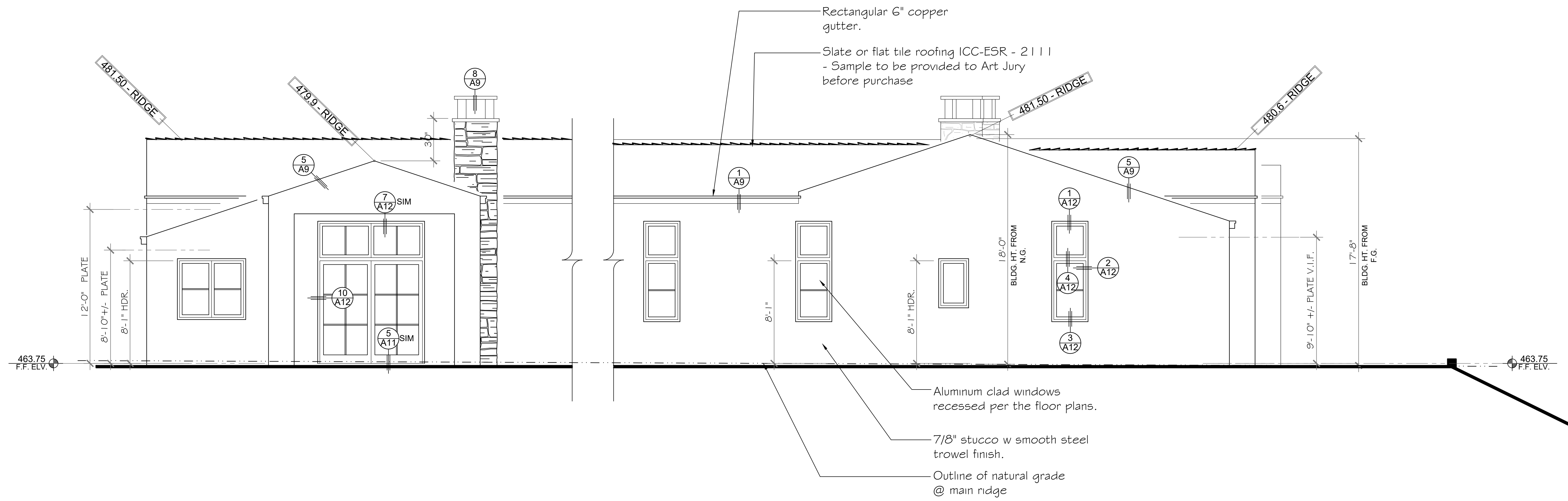
REAR SOUTH ELEVATION 1/4" = 1'-0"
