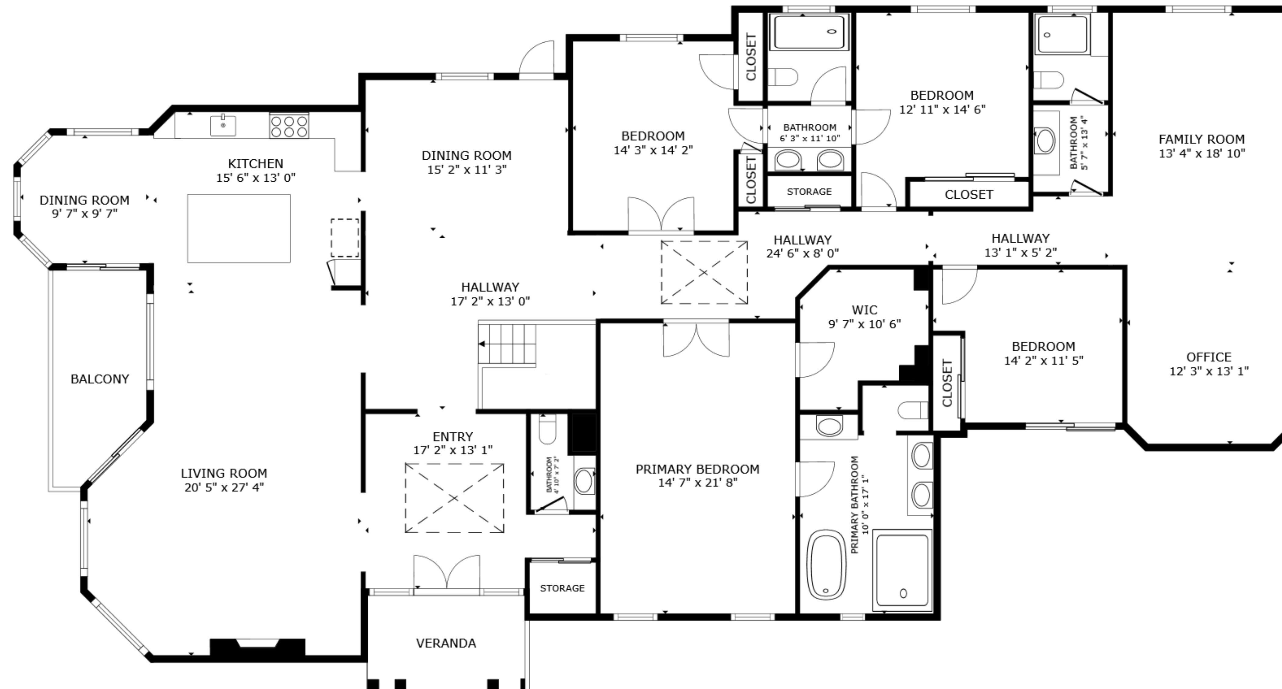
FLOOR 2
