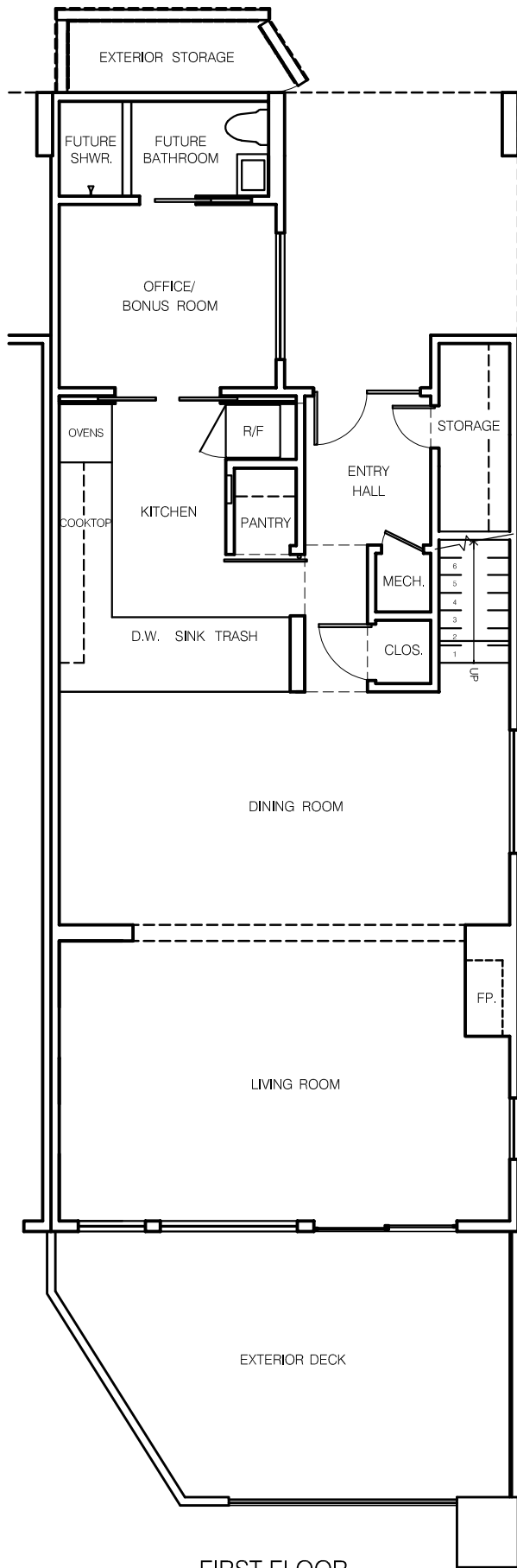
FIRST FLOOR NOT TO SCALE 736 GOULD AVENUE #33 HERMOSA BEACH, CA 90254
