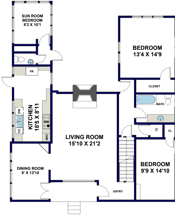
MIDDLE LEVEL
