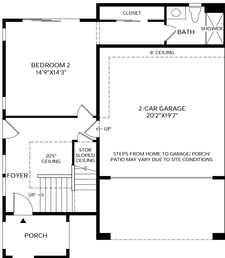
FIRST FLOOR 9' CEILING HEIGHT
