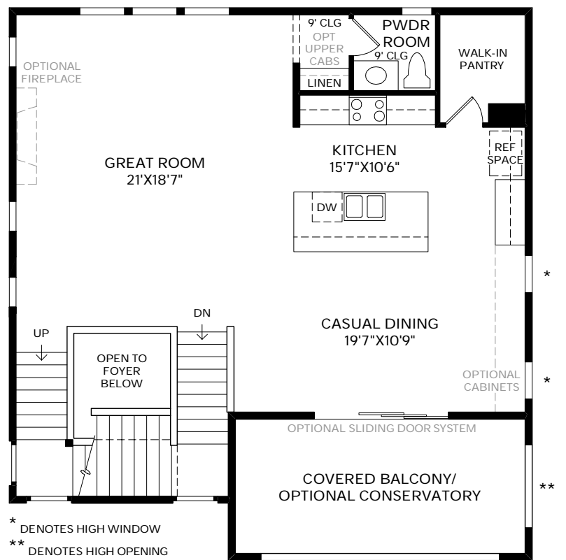
SECOND FLOOR 10' CEILING HEIGHT
