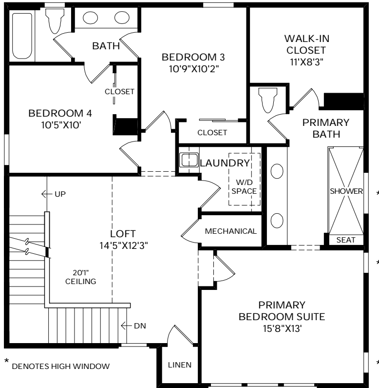
THIRD FLOOR 9' CEILING HEIGHT
