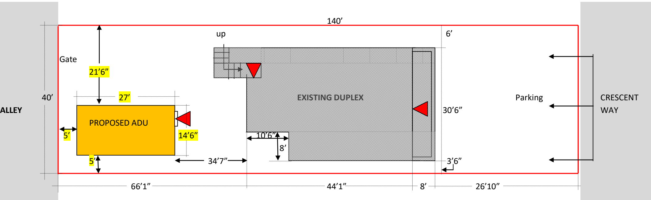
PLOT PLAN Scale - 1":16'0"
