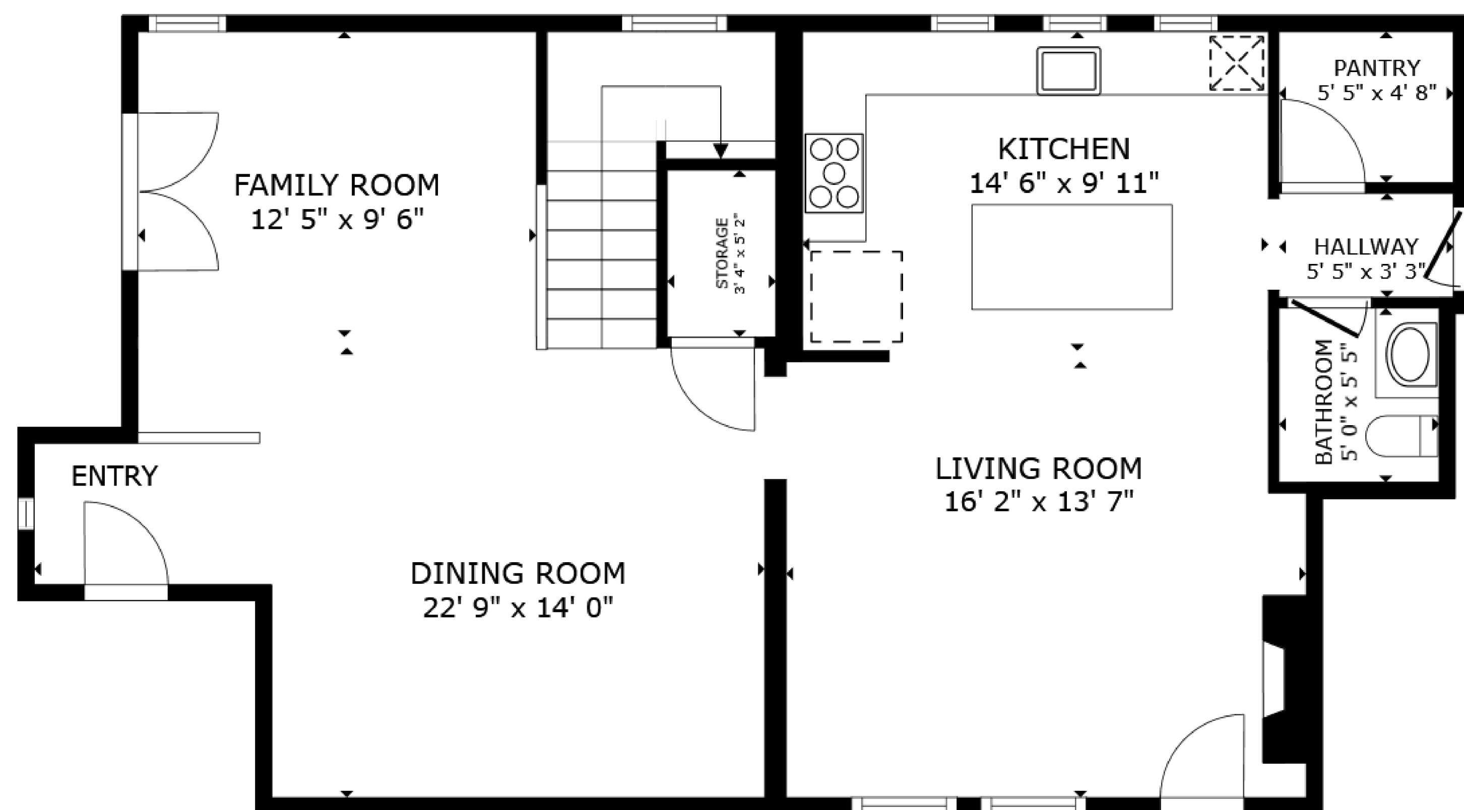
FLOOR 1
