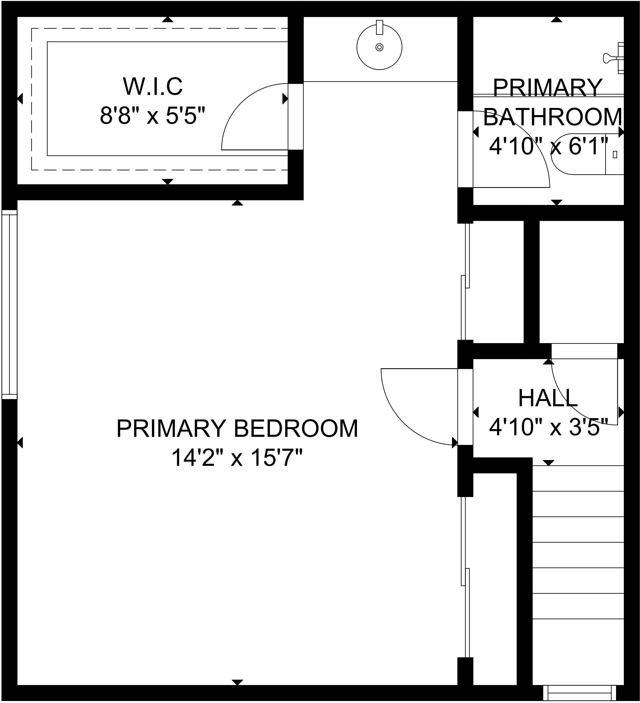
FLOOR 2
