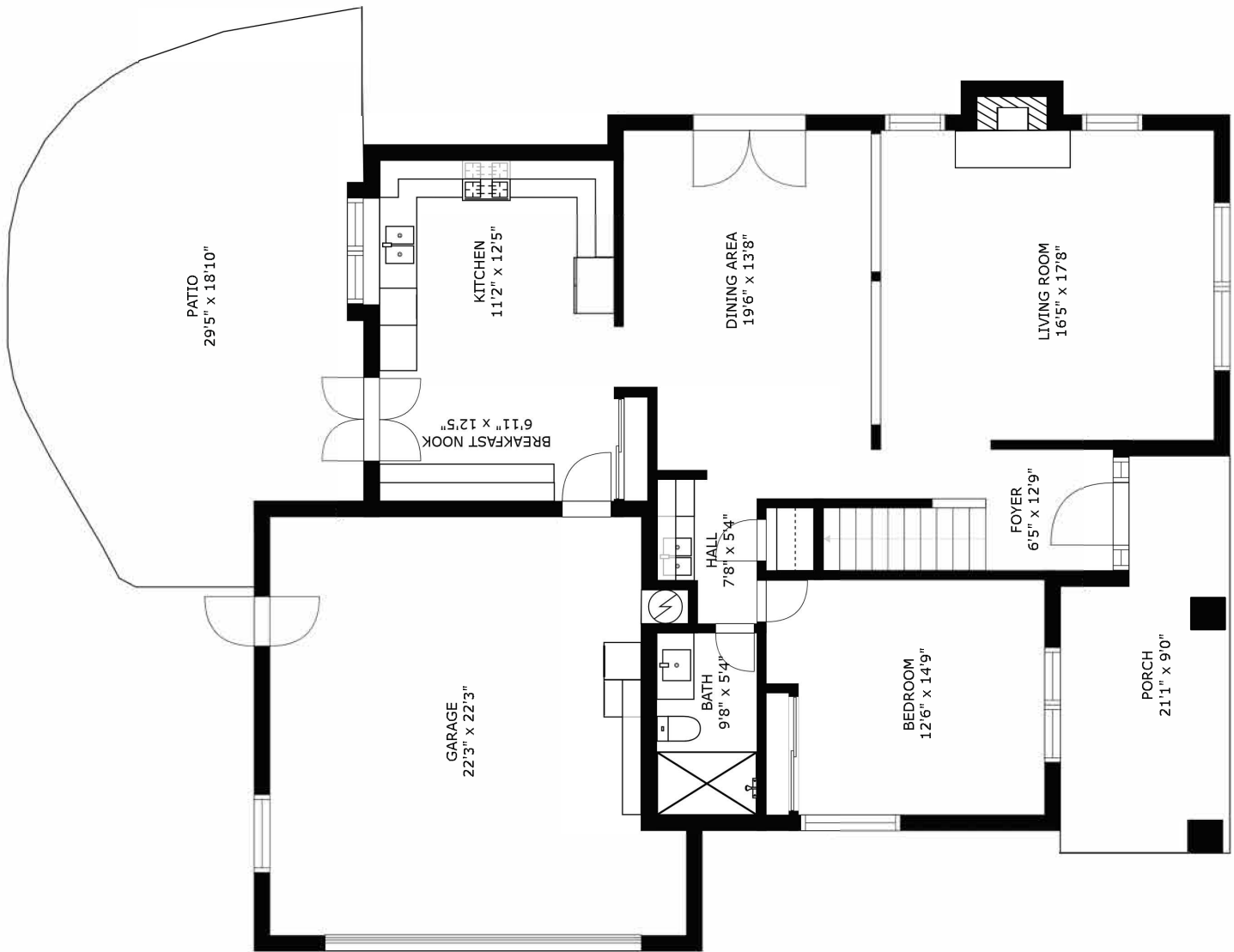
FLOOR 1
