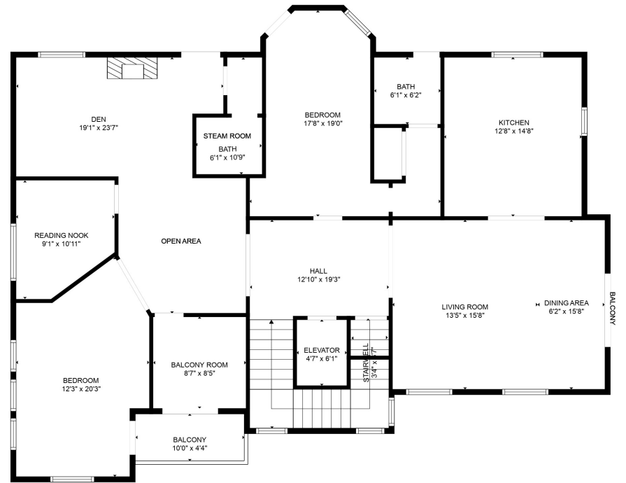
FLOOR 3
