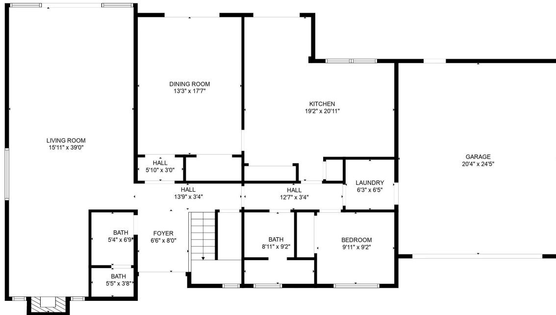
FLOOR 1
