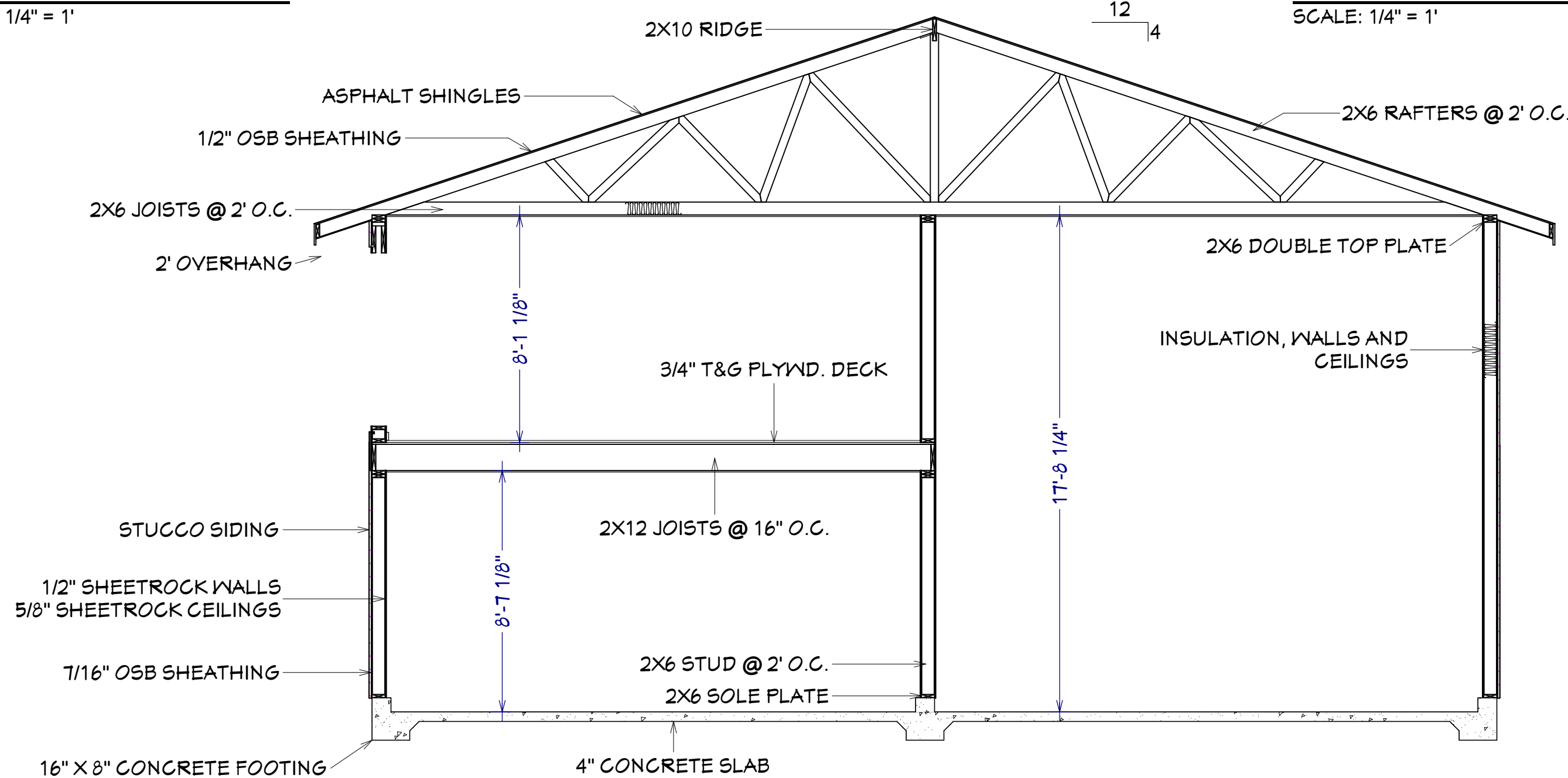
40x42 House #40X42H1C
