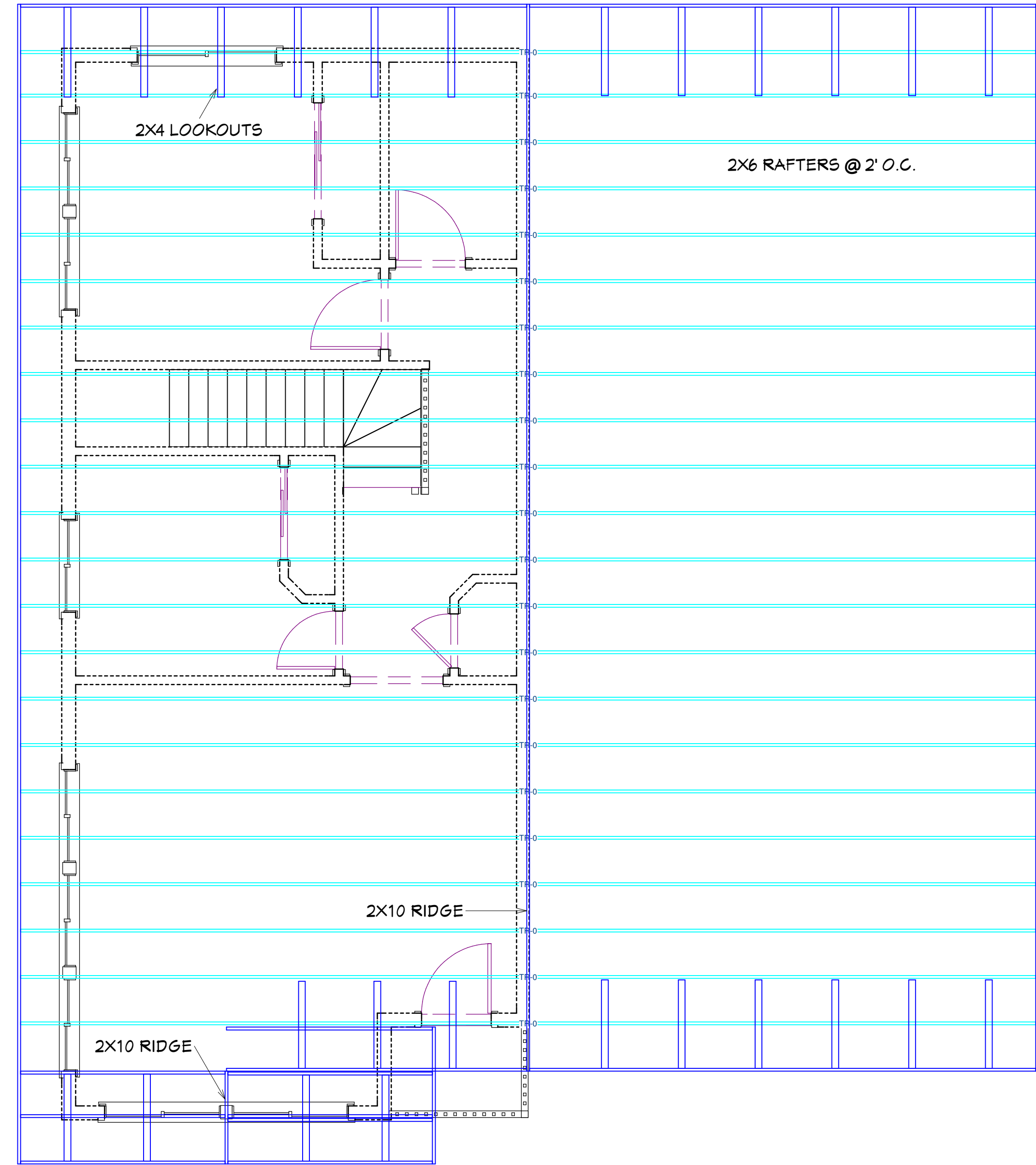
ROOF FRAMING PLAN SCALE: 1/4" = 1'
