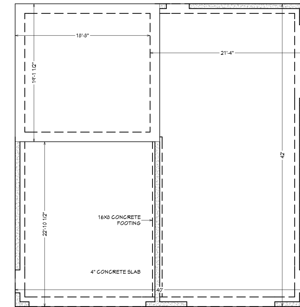
FOUNDATION PLAN SCALE: 1/8" = 1'
