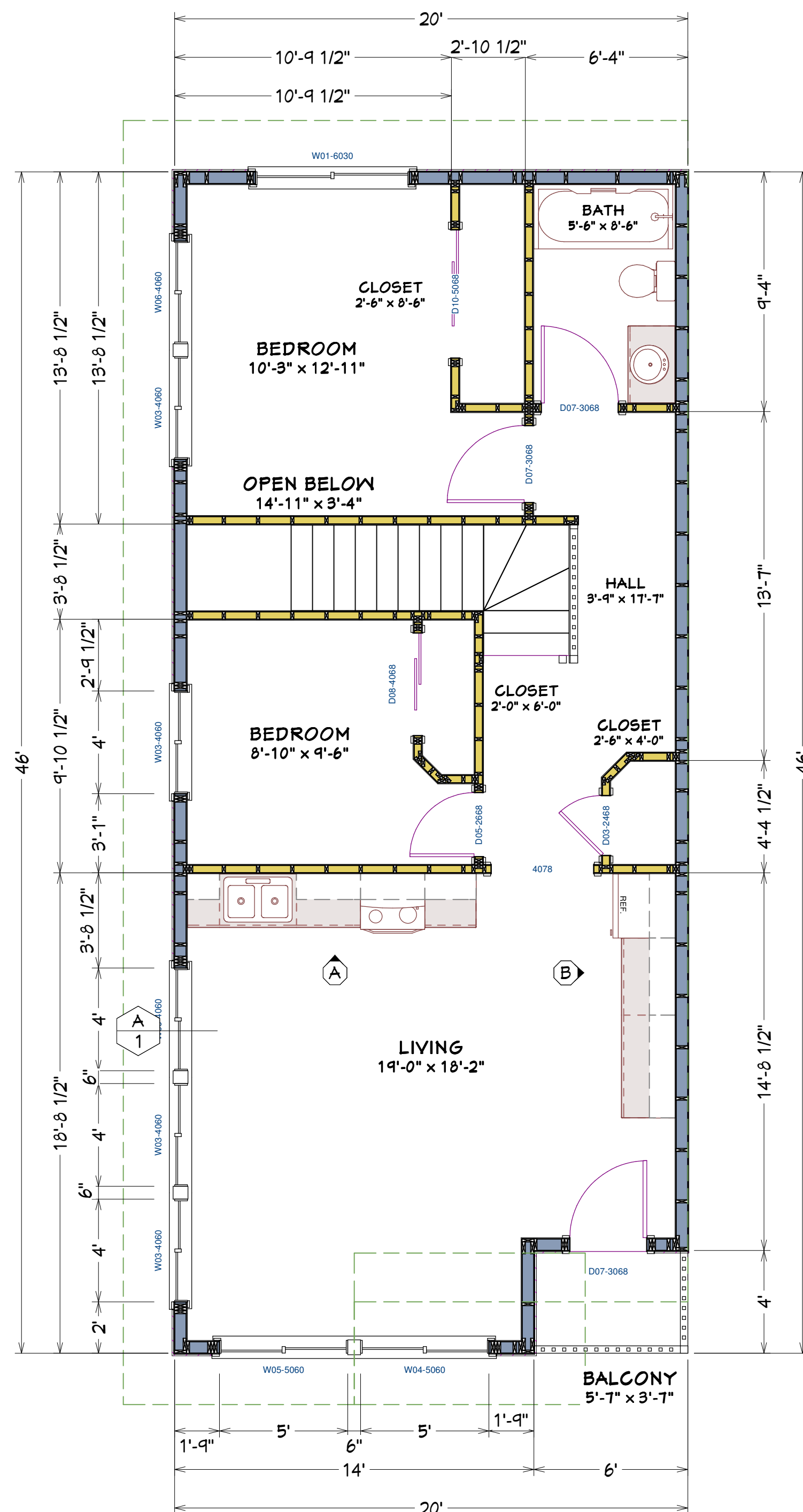
2ND FLOOR PLAN SCALE: 1/4" = 1'
