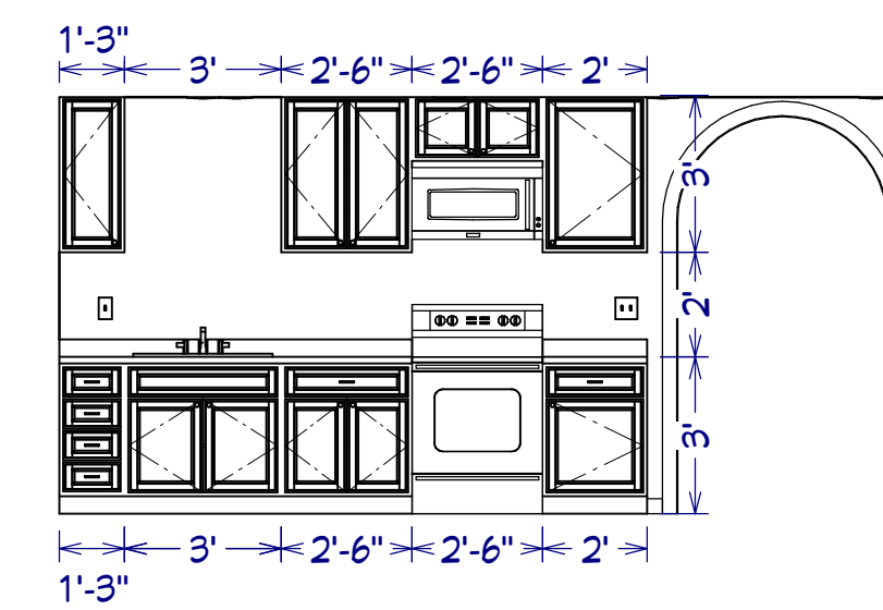
CABINET ELEVATION A SCALE: 1/4" = 1'
