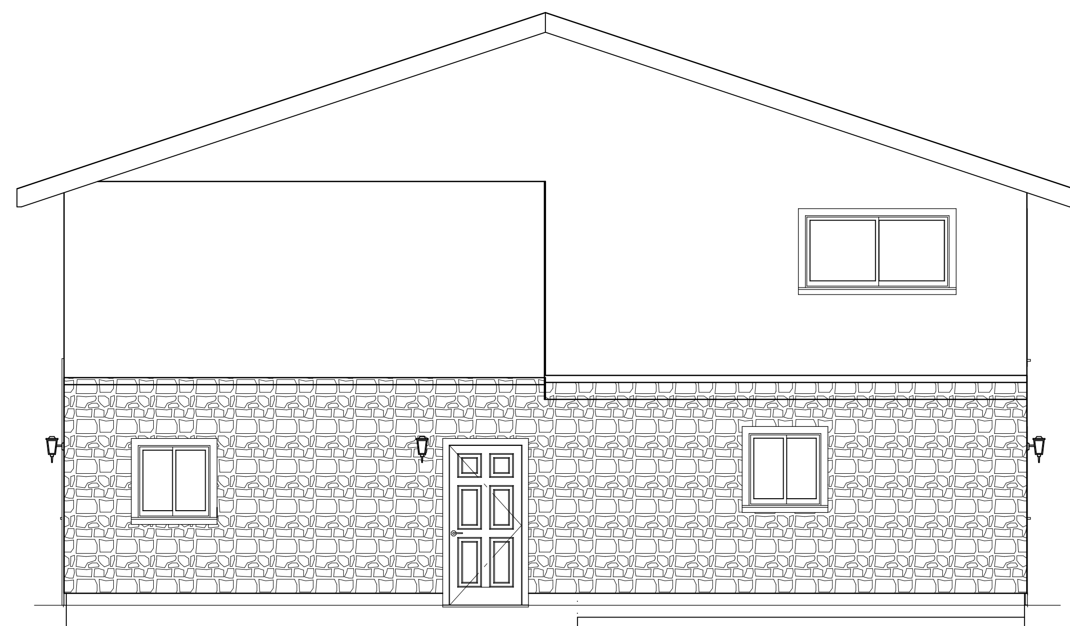
FRONT ELEVATION SCALE: 1/4" = 1'
