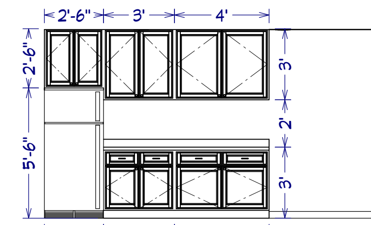
CABINET ELEVATION B SCALE: 1/4" = 1'
