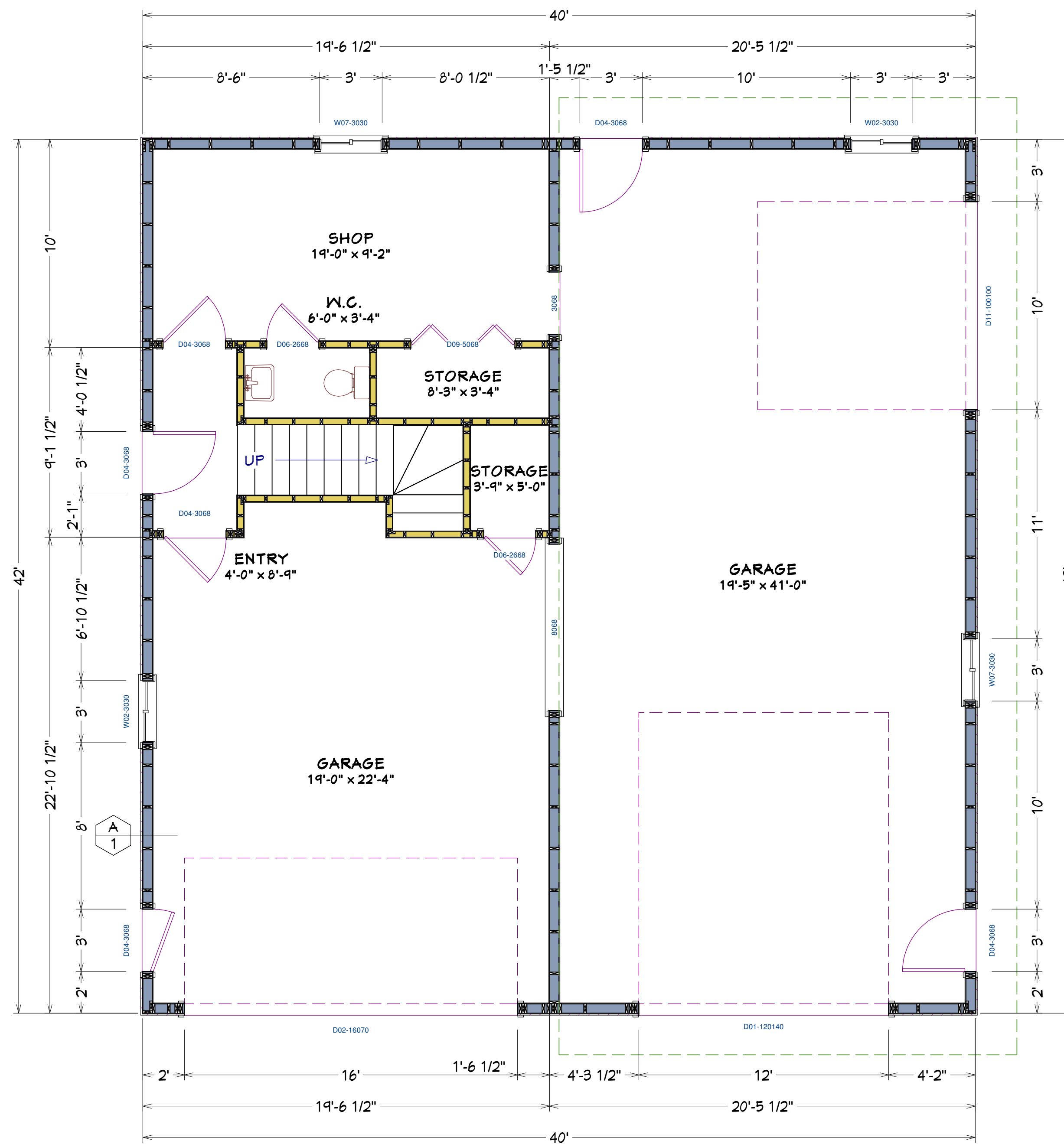
MAIN FLOOR PLAN SCALE: 1/4" = 1'
