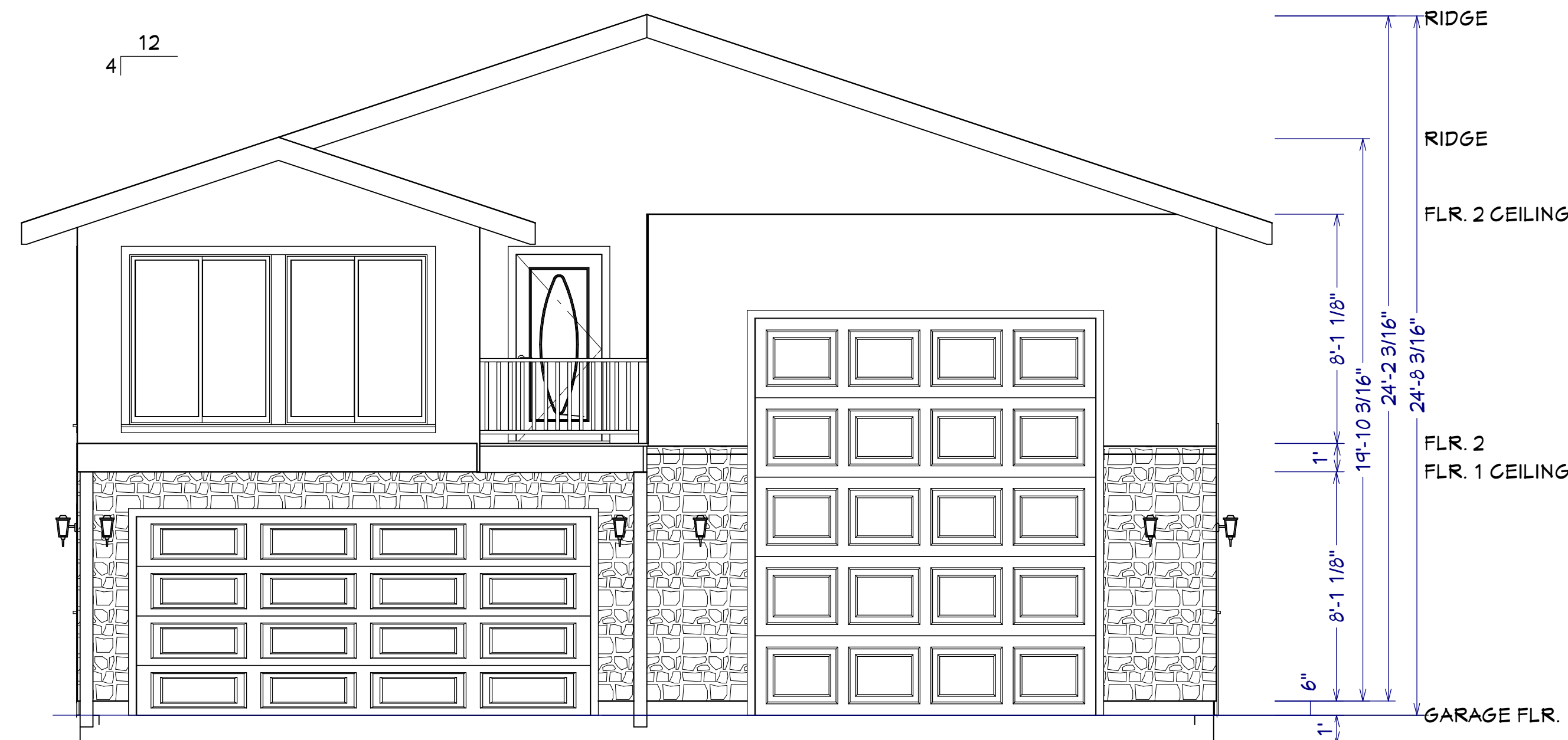
FRONT ELEVATION SCALE: 1/4" = 1'
