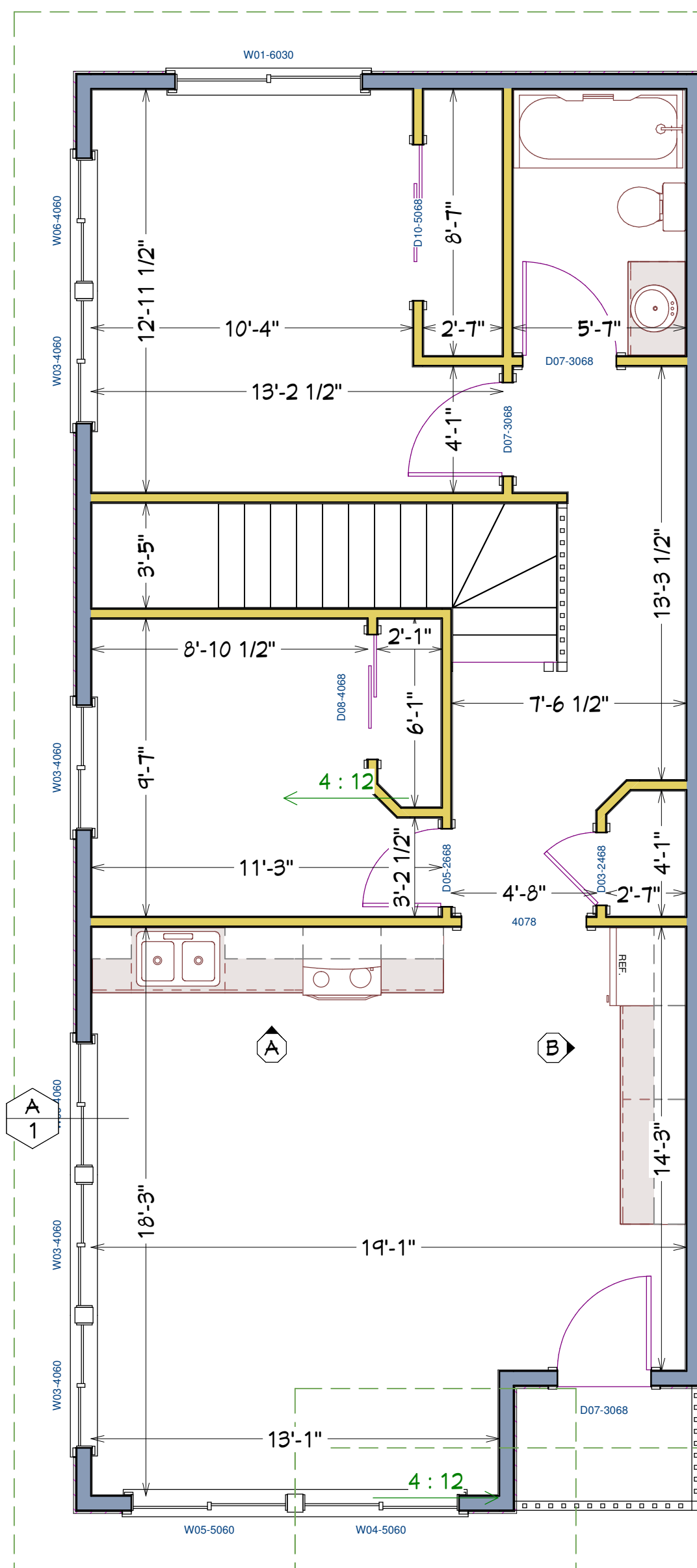
2ND FLOOR PLAN SCALE: 1/4" = 1'
