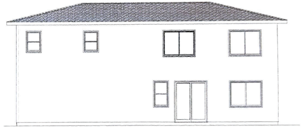
SOUTH ELEVATION
