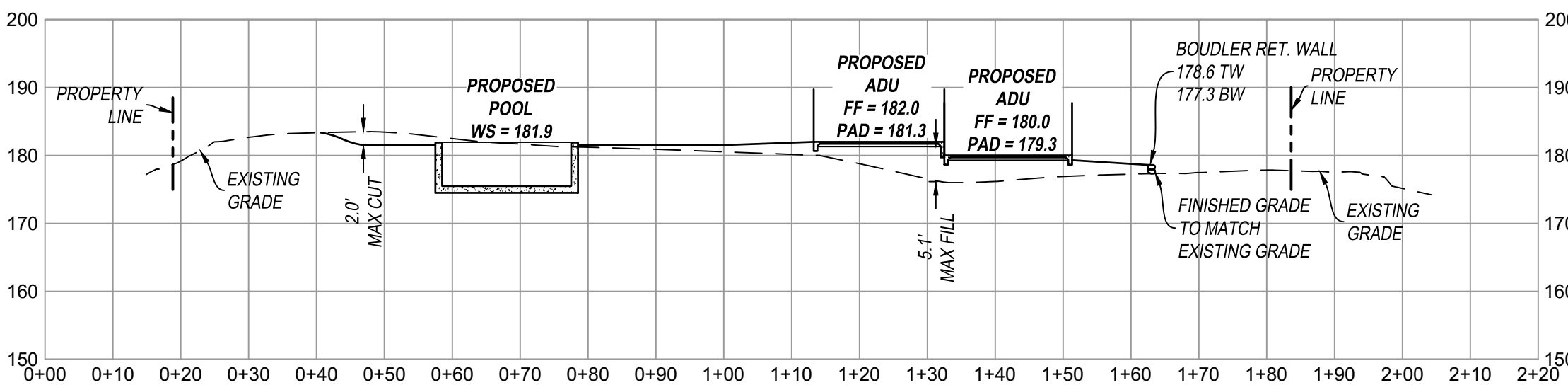
SECTION C-C 1" = 20'
