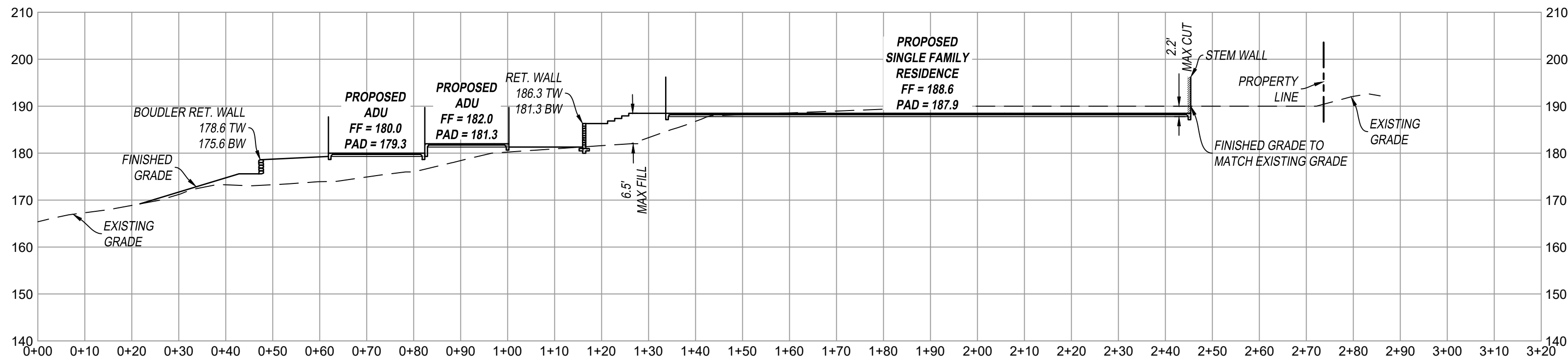
SECTION A-A 1" = 20'
