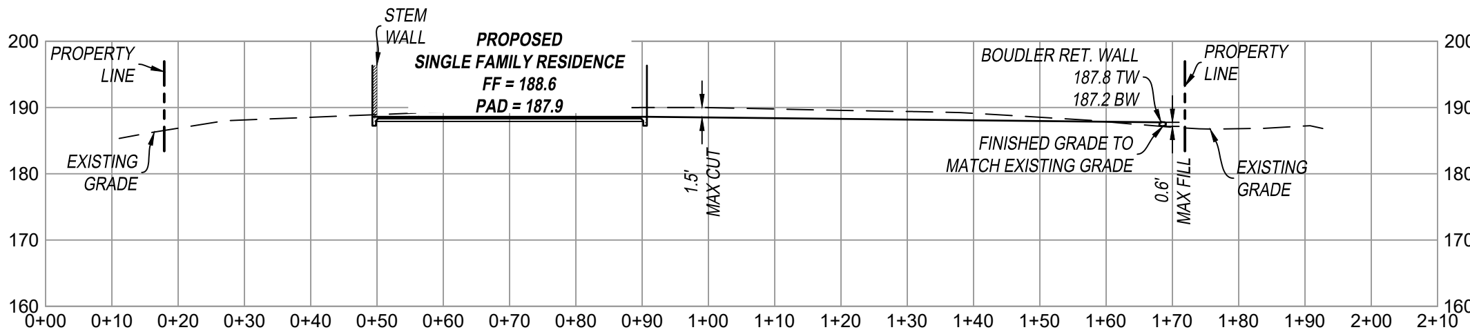
SECTION B-B 1" = 20'
