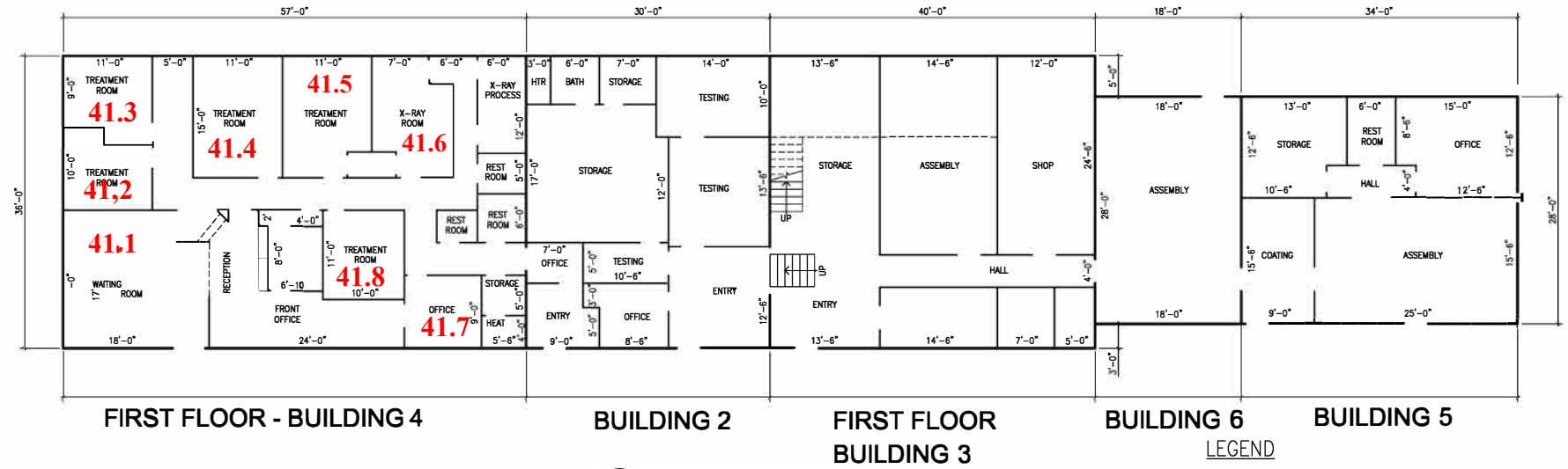
2 OCCUPANCY PLANS 1/8" = 1'-0"
