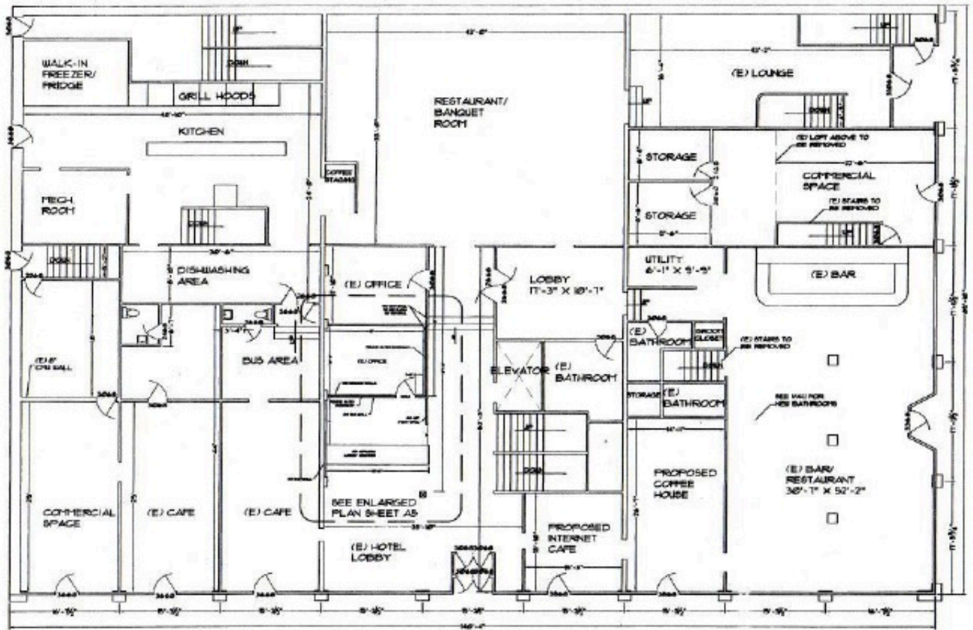
HOTEL MT. LASSEN MAIN FLOOR PLAN SCALE 3/8" = 1'-0"
