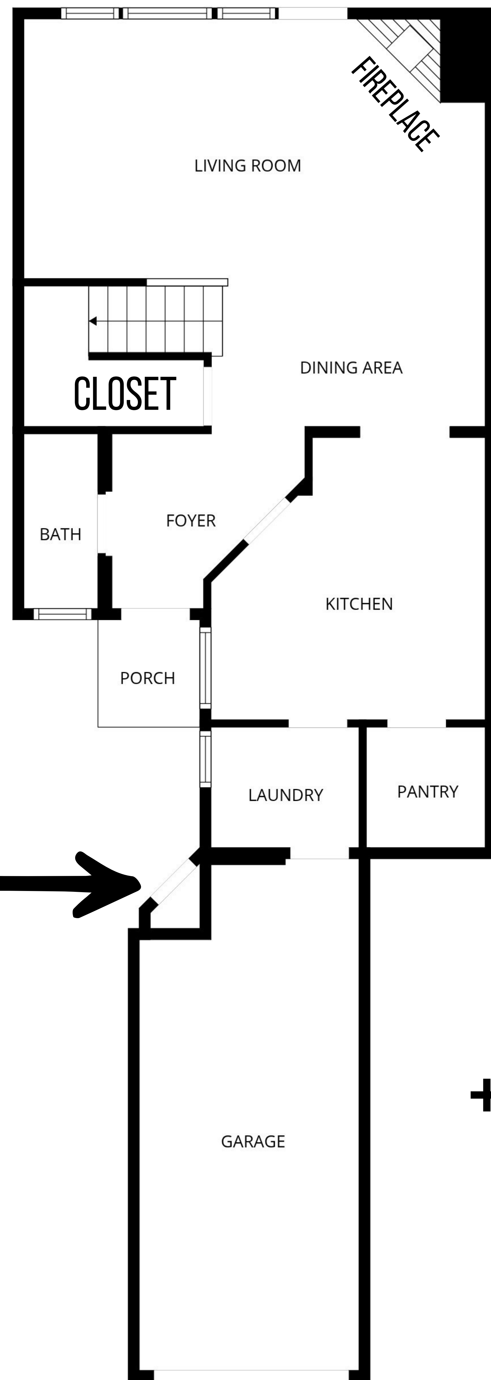
1st floor
