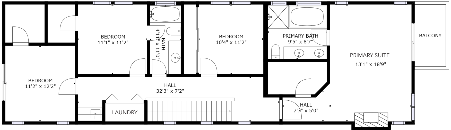
FLOOR 2
