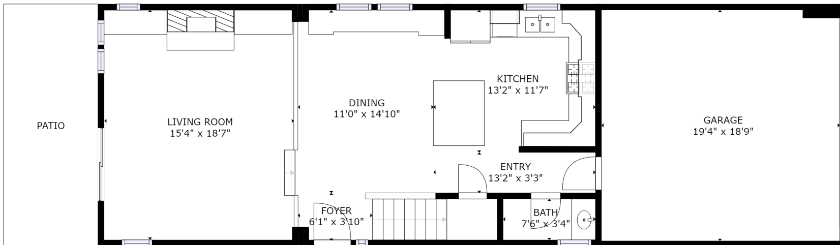
FLOOR 1
