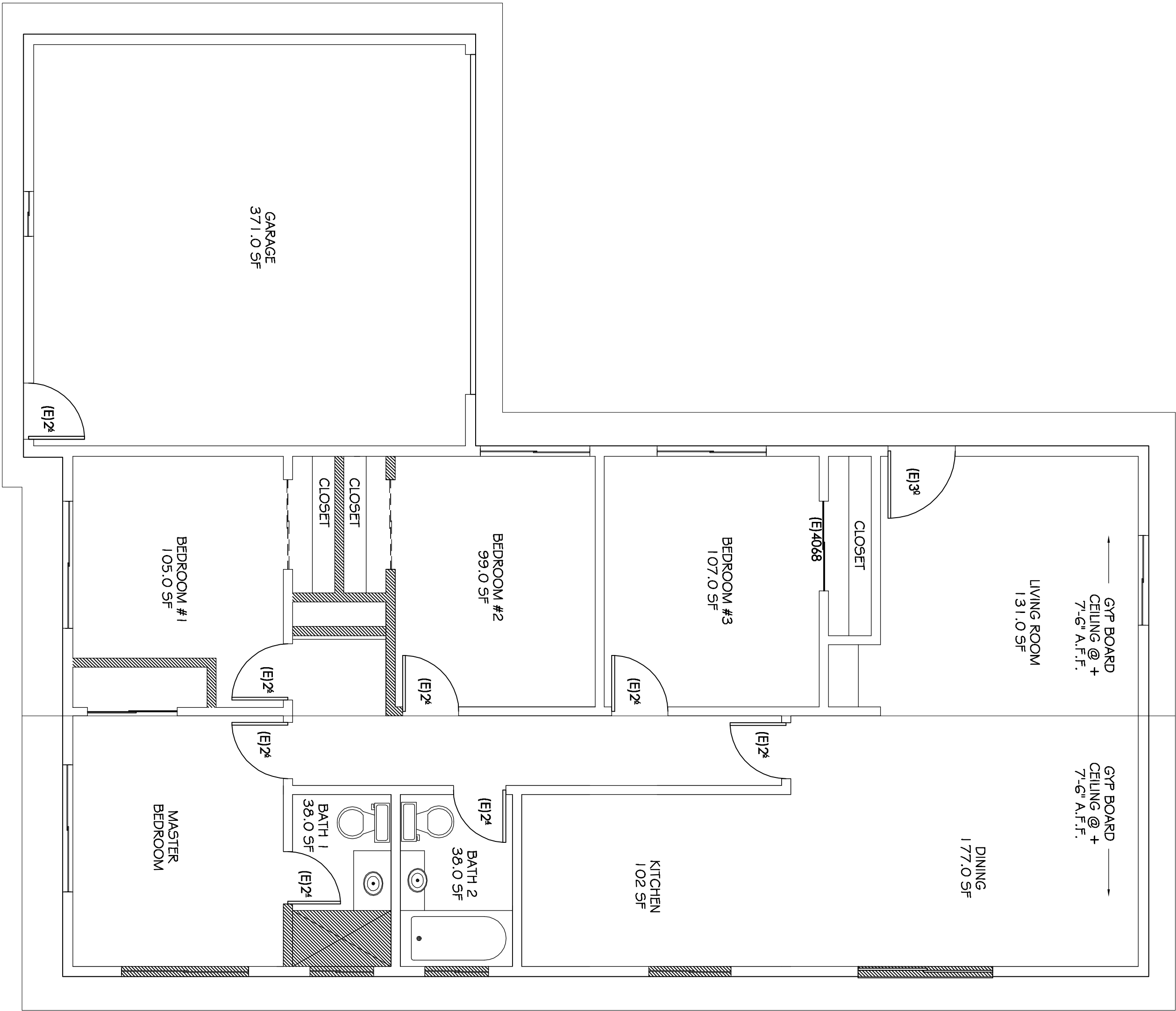
(E) FLOOR PLAN
