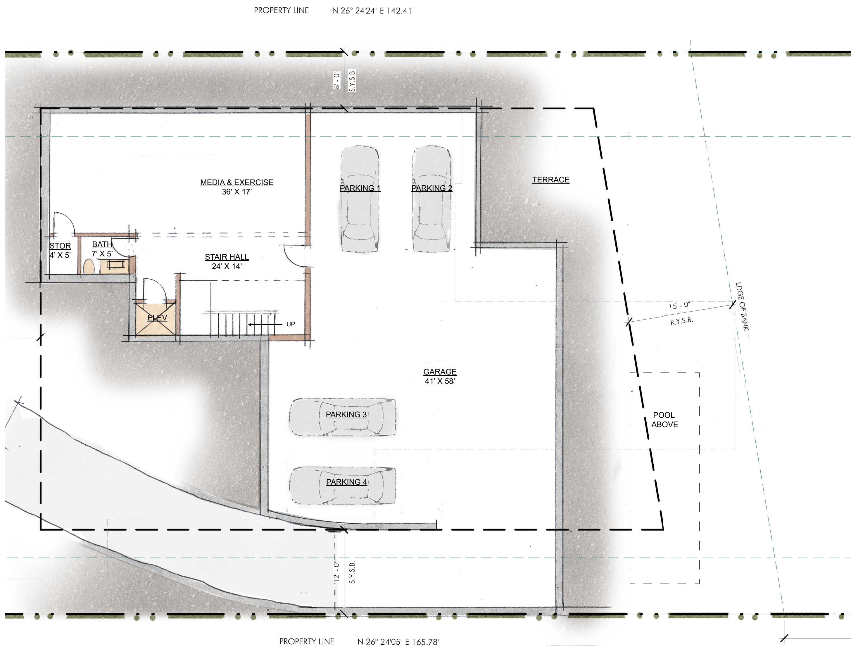
LOWER LEVEL PLAN SCALE 1/8" = 1'-0"
