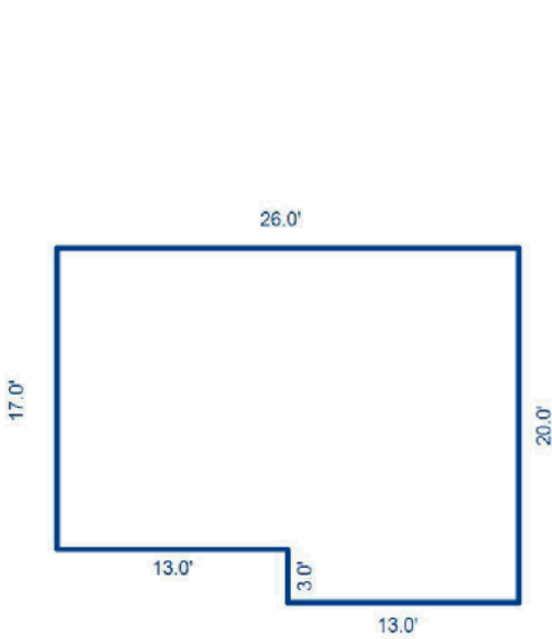
SECOND FLOOR
