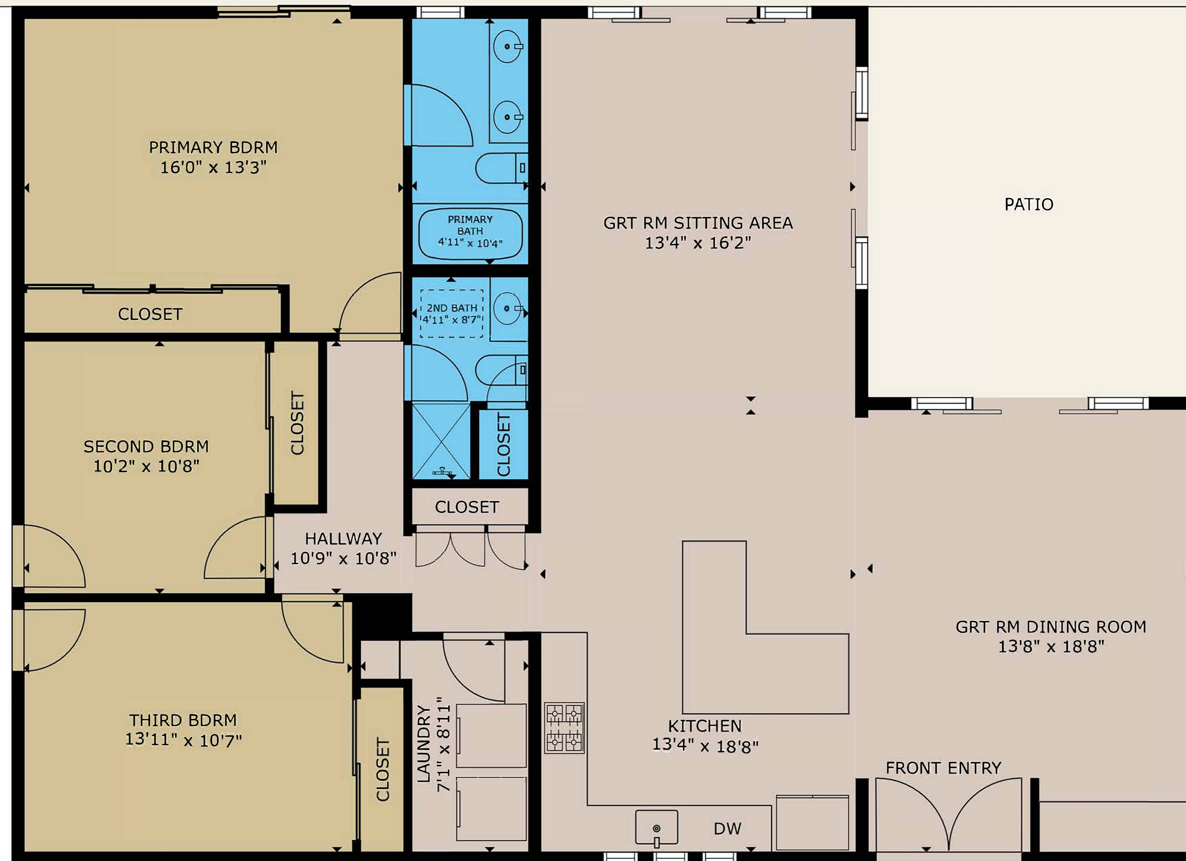
FLOOR PLAN
